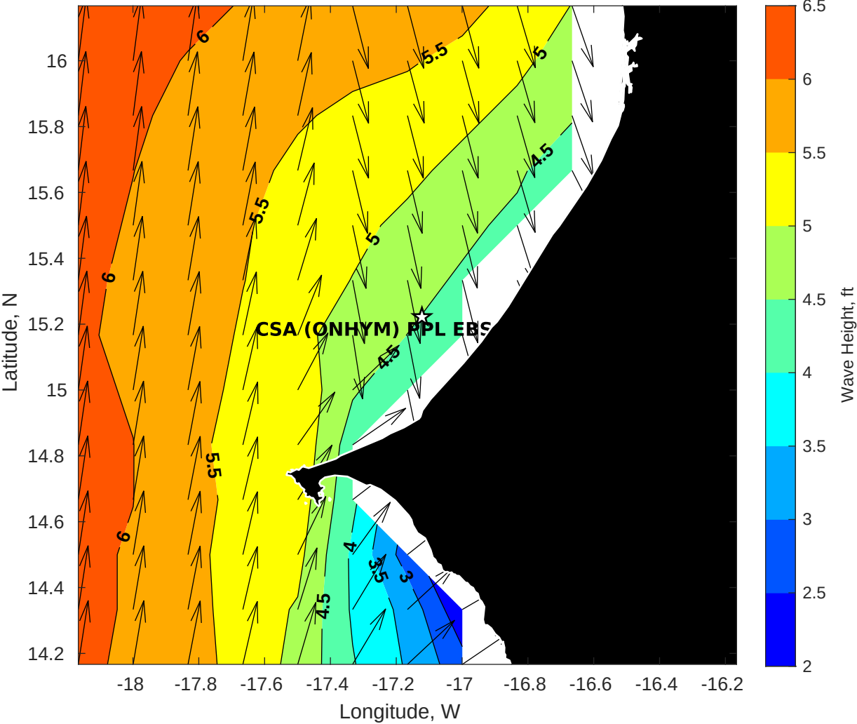
Wave Height (ft) for CSA (ONHYM) PPL EBS - Senegal at 19-Jun-2025 09:00:00
