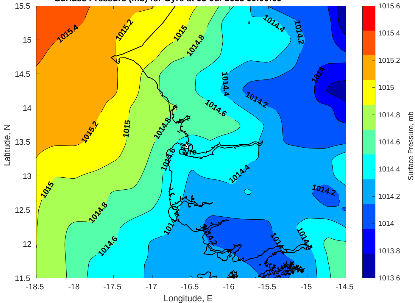
Surface Pressure (mb) for Gyre at 05-Jul-2025 00:00:00
