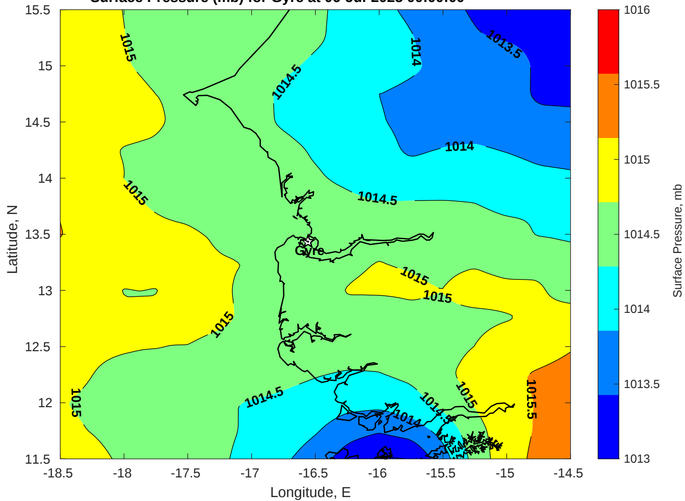
Surface Pressure (mb) for Gyre at 06-Jul-2025 00:00:00
