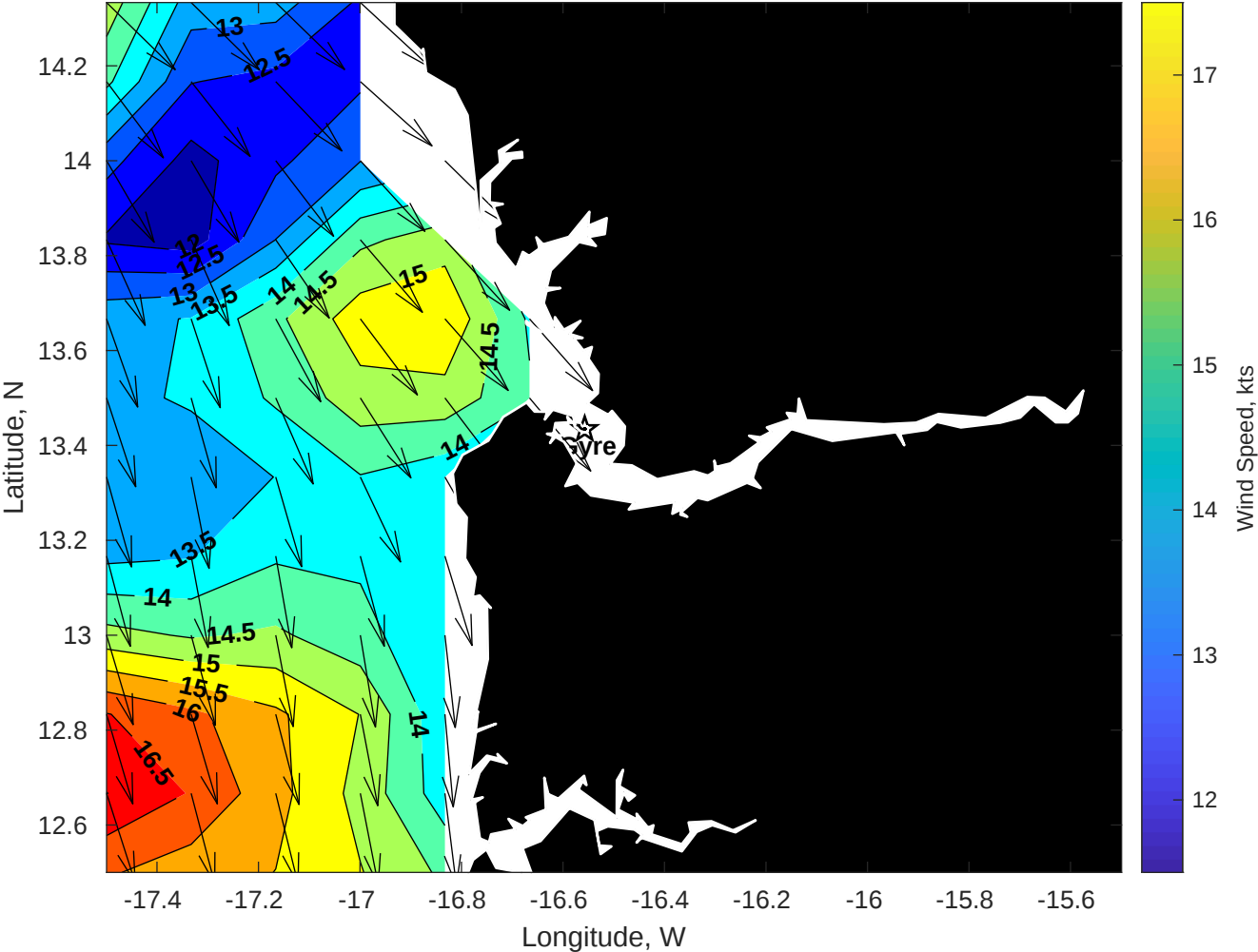
Winds (kts) for Gyre at 05-Jul-2025 09:00:00
