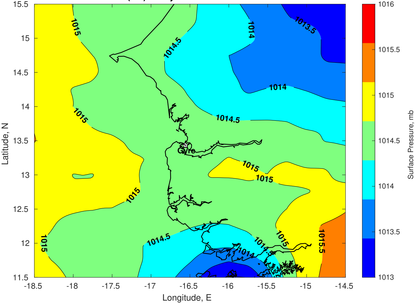
Surface Pressure (mb) for Gyre at 06-Jul-2025 00:00:00
