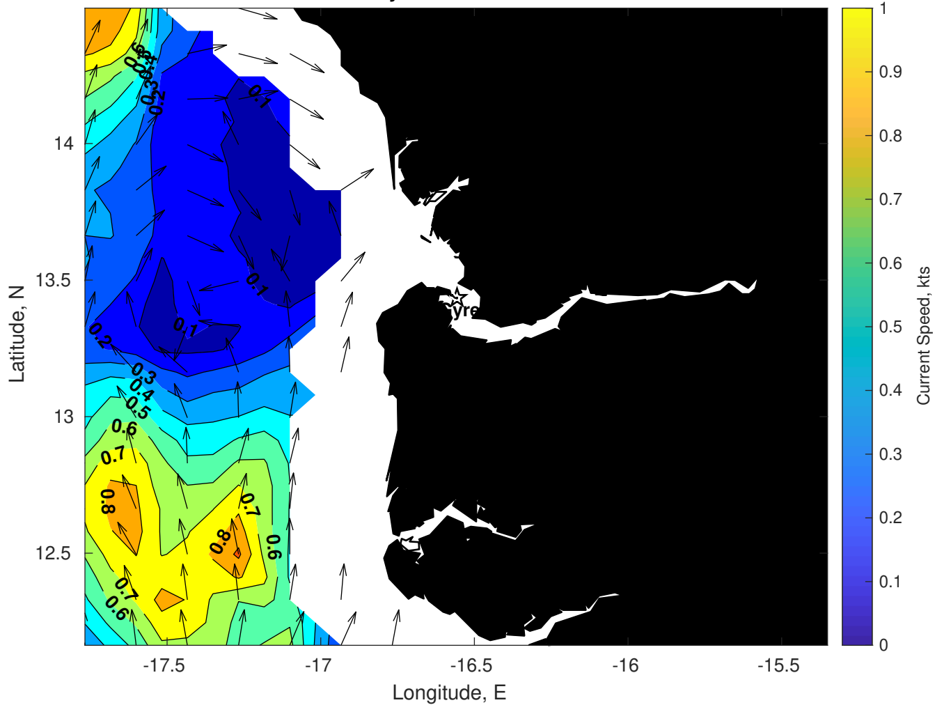
Surface Currents for Gyre at 04-Jul-2025 00:00:00
