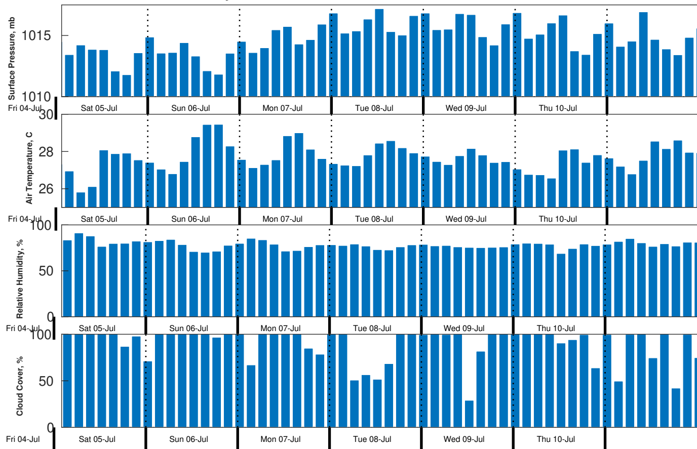
Met Forecast for Gyre from 04-Jul-2025 23:00:00 to 11-Jul-2025 23:00:00
