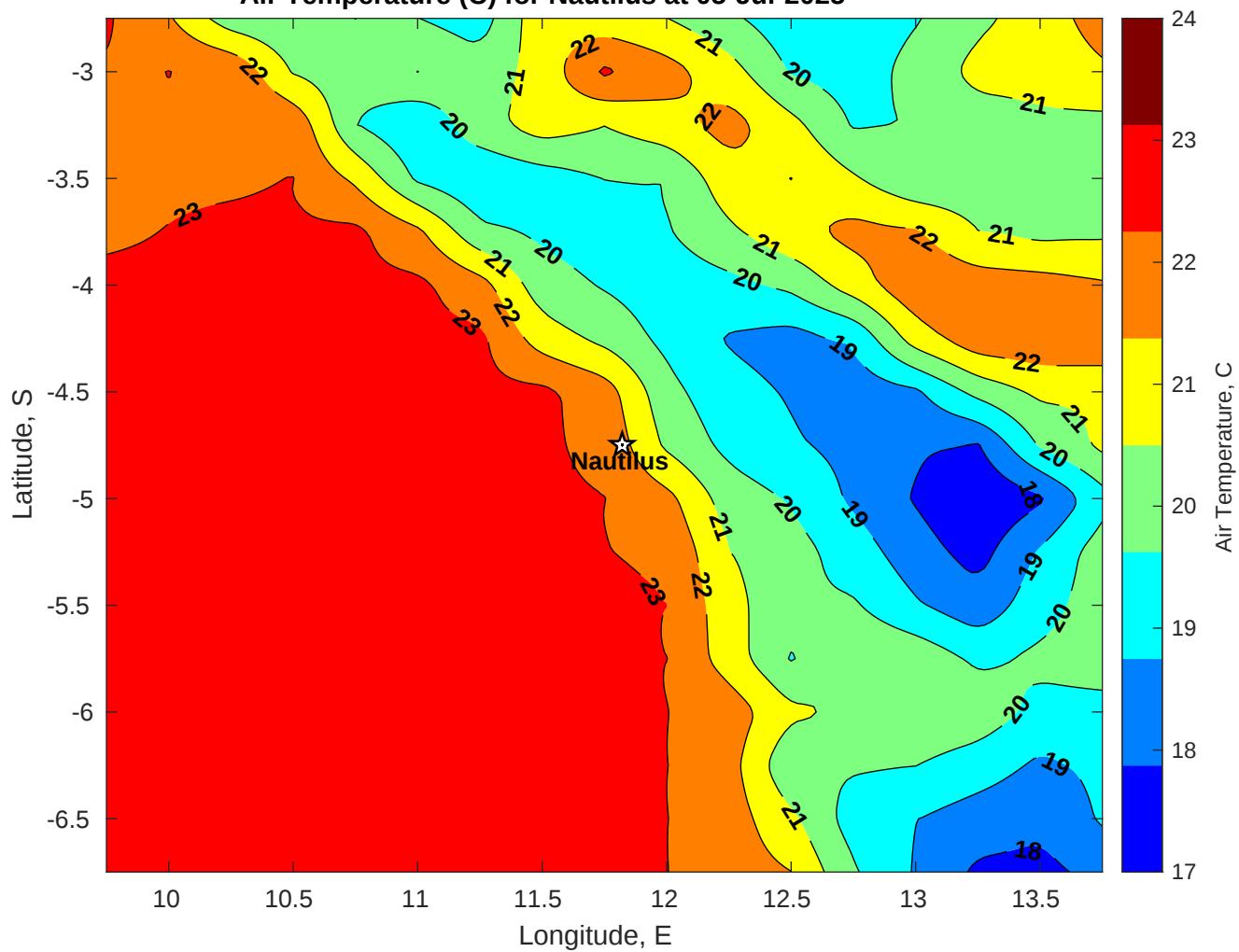
Air Temperature (C) for Nautilus at 05-Jul-2025
