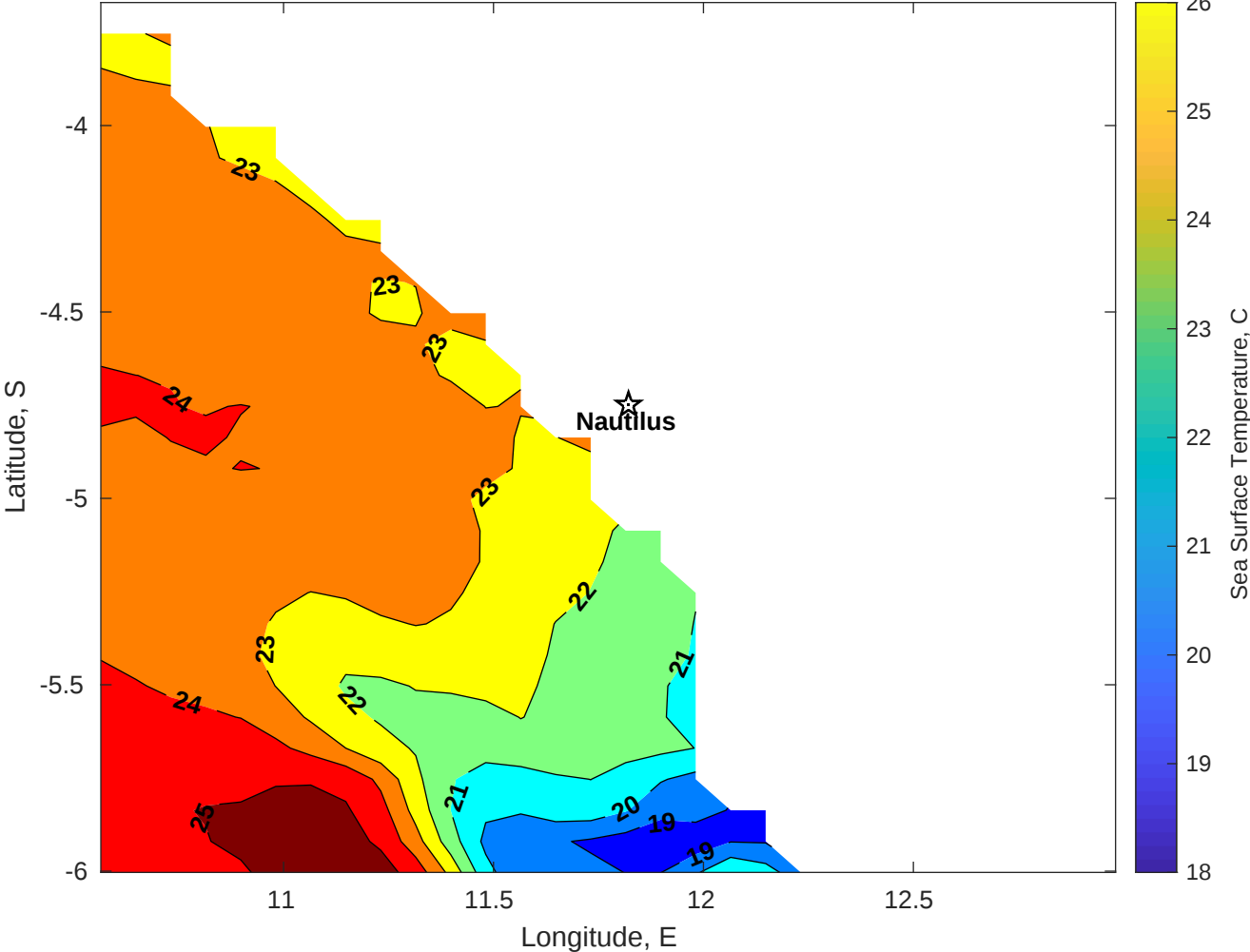
SST for Nautilus at 04-Jul-2025 00:00:00
