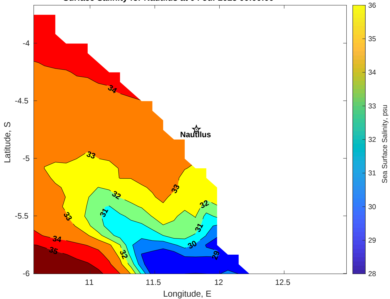
Surface Salinity for Nautilus at 04-Jul-2025 00:00:00
