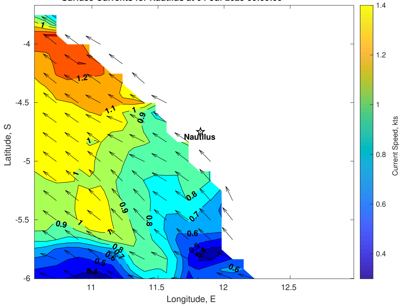
Surface Currents for Nautilus at 04-Jul-2025 00:00:00
