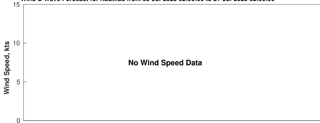
Wind & Wave Forecast for Nautilus from 05-Jul-2025 02:00:00 to 21-Jul-2025 02:00:00
