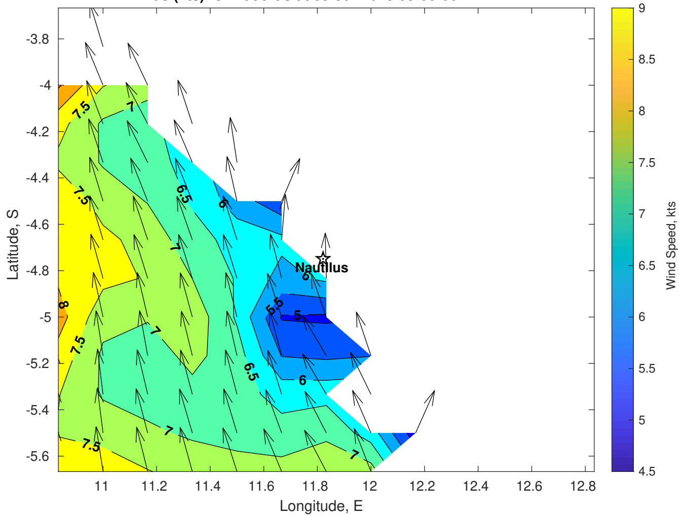
Winds (kts) for Nautilus at 05-Jul-2025 09:00:00
