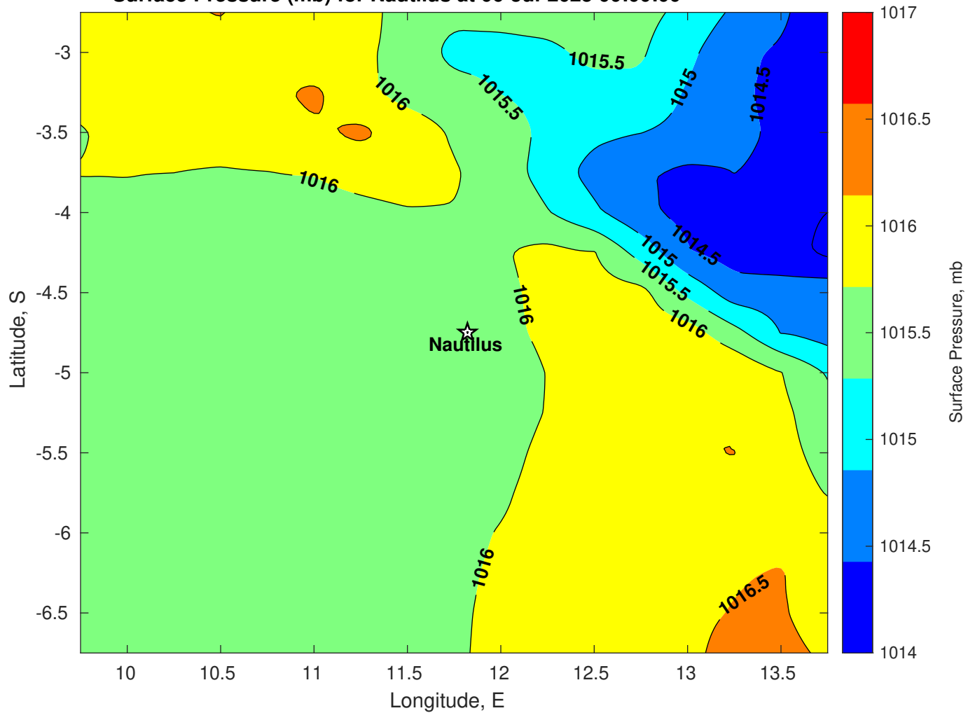
Surface Pressure (mb) for Nautilus at 06-Jul-2025 00:00:00
