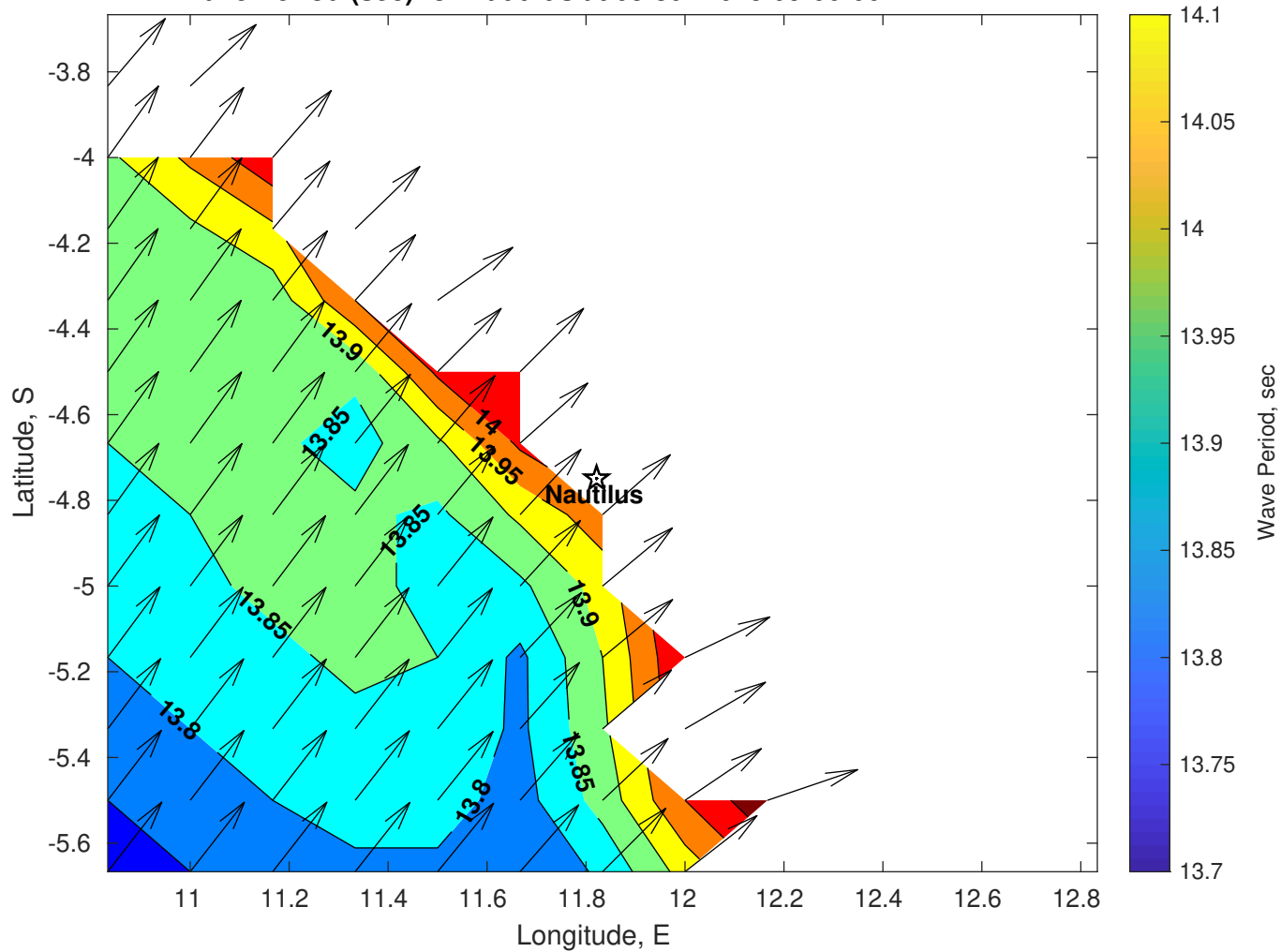
Wave Period (sec) for Nautilus at 05-Jul-2025 09:00:00
