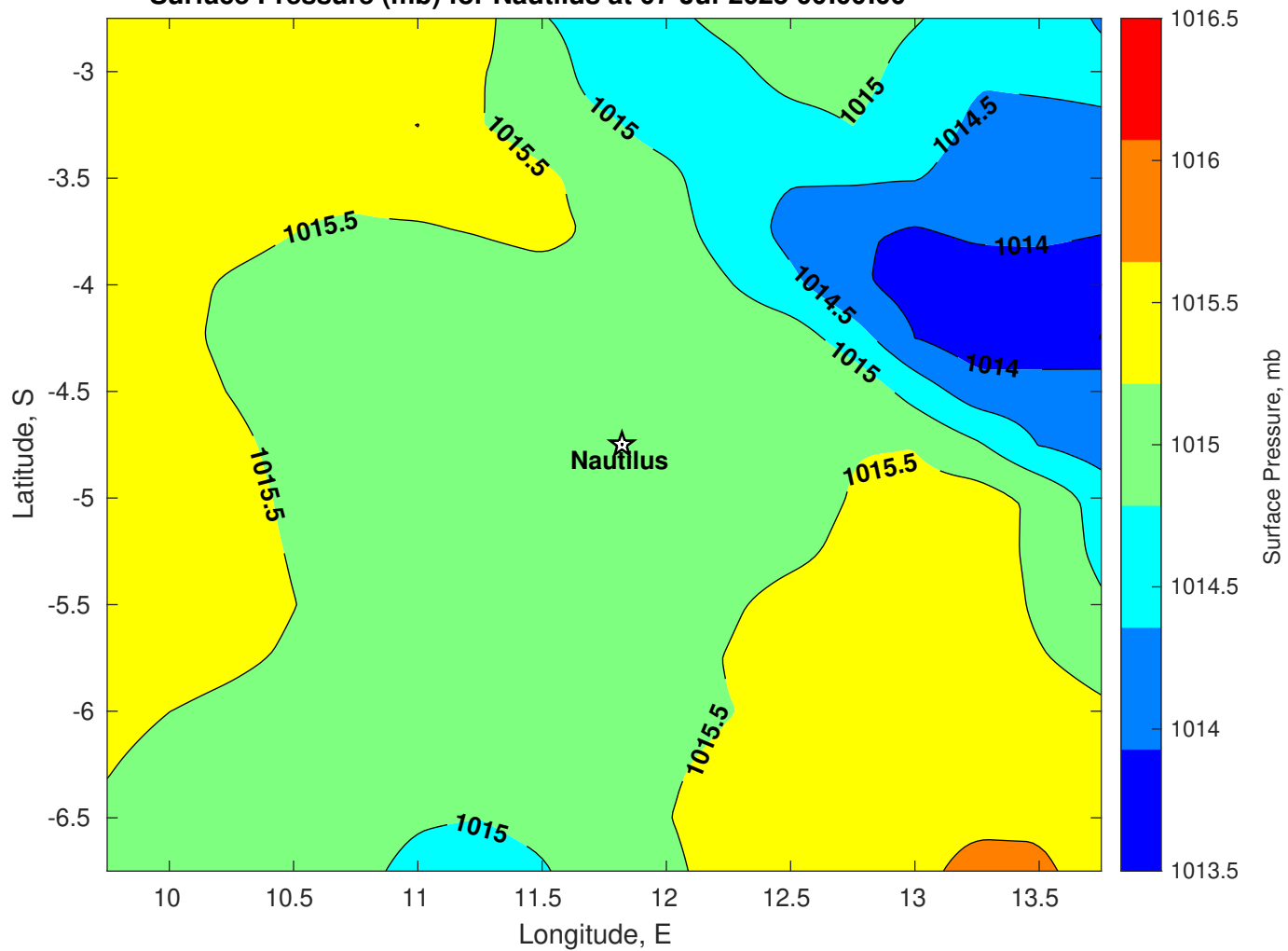
Surface Pressure (mb) for Nautilus at 07-Jul-2025 00:00:00
