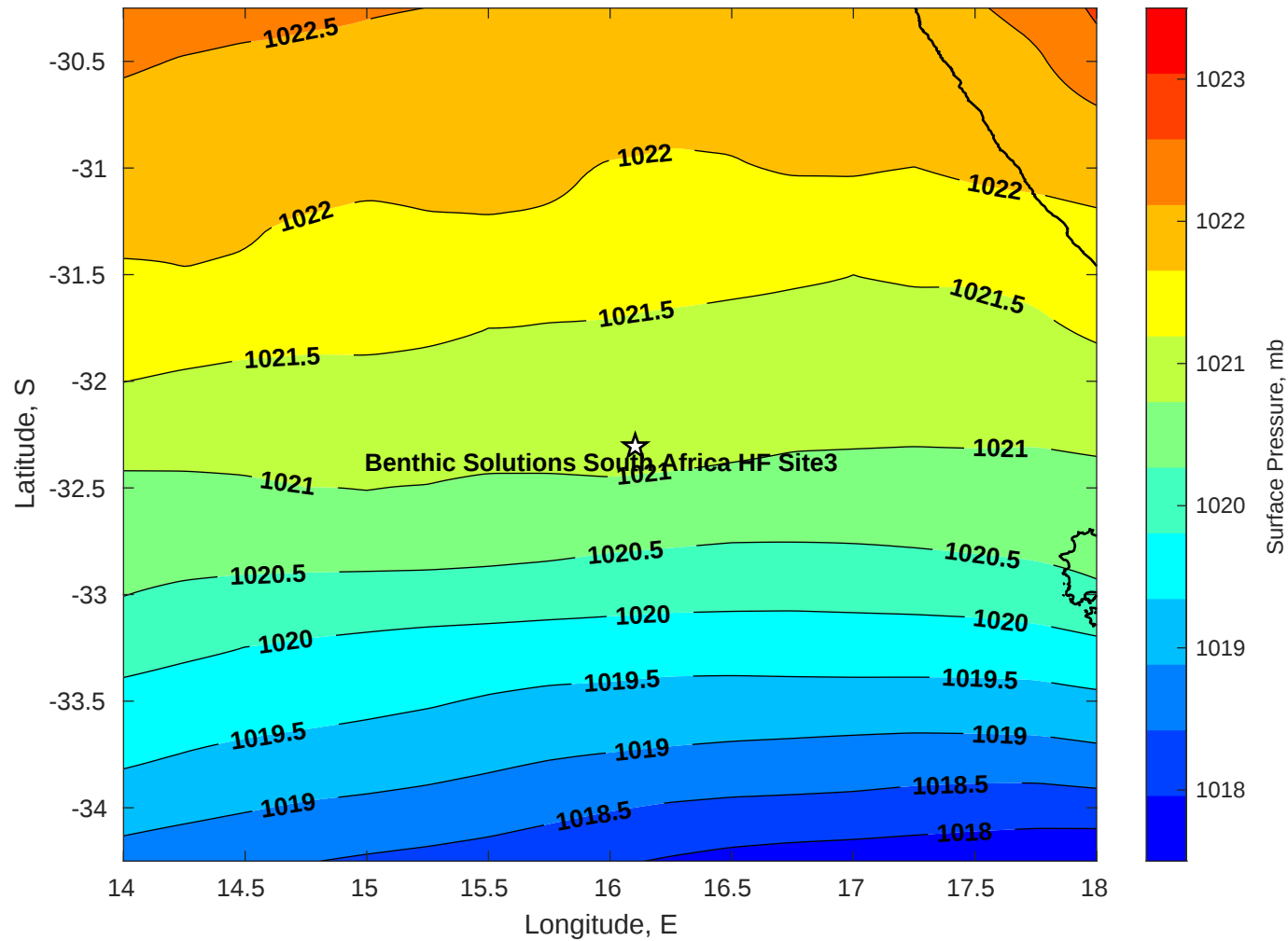
Surface Pressure (mb) for Benthic Solutions South Africa HF Site3 at 20-Jun-2025 00:00:00
