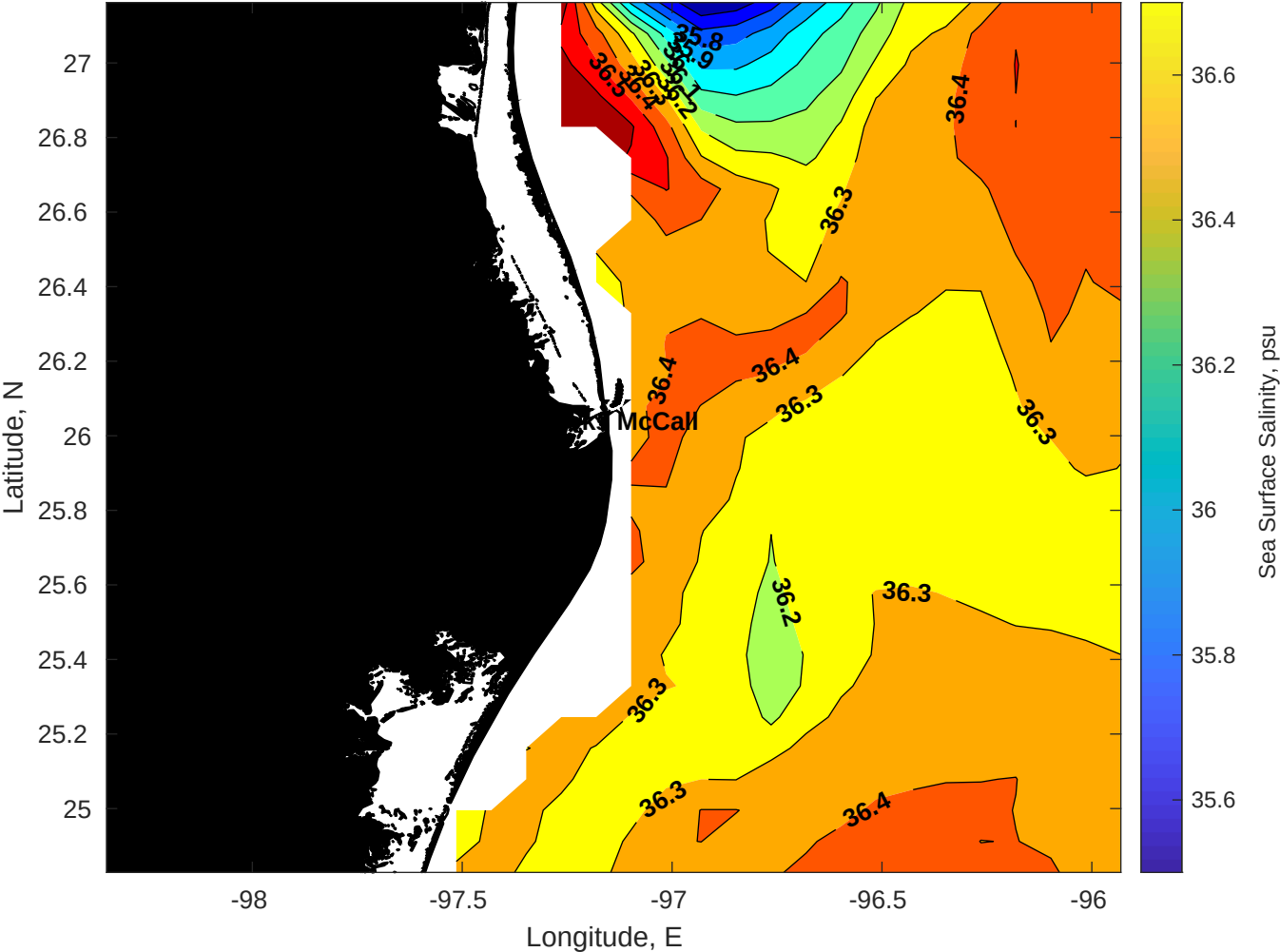
Surface Salinity for Brooks McCall at 05-Jul-2025 00:00:00
