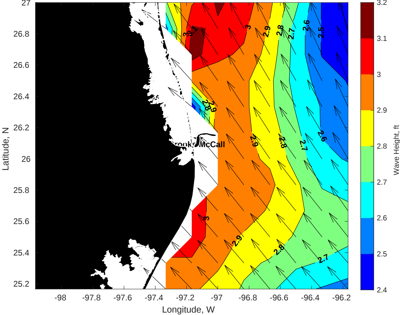
Wave Height (ft) for Brooks McCall at 06-Jul-2025 09:00:00
