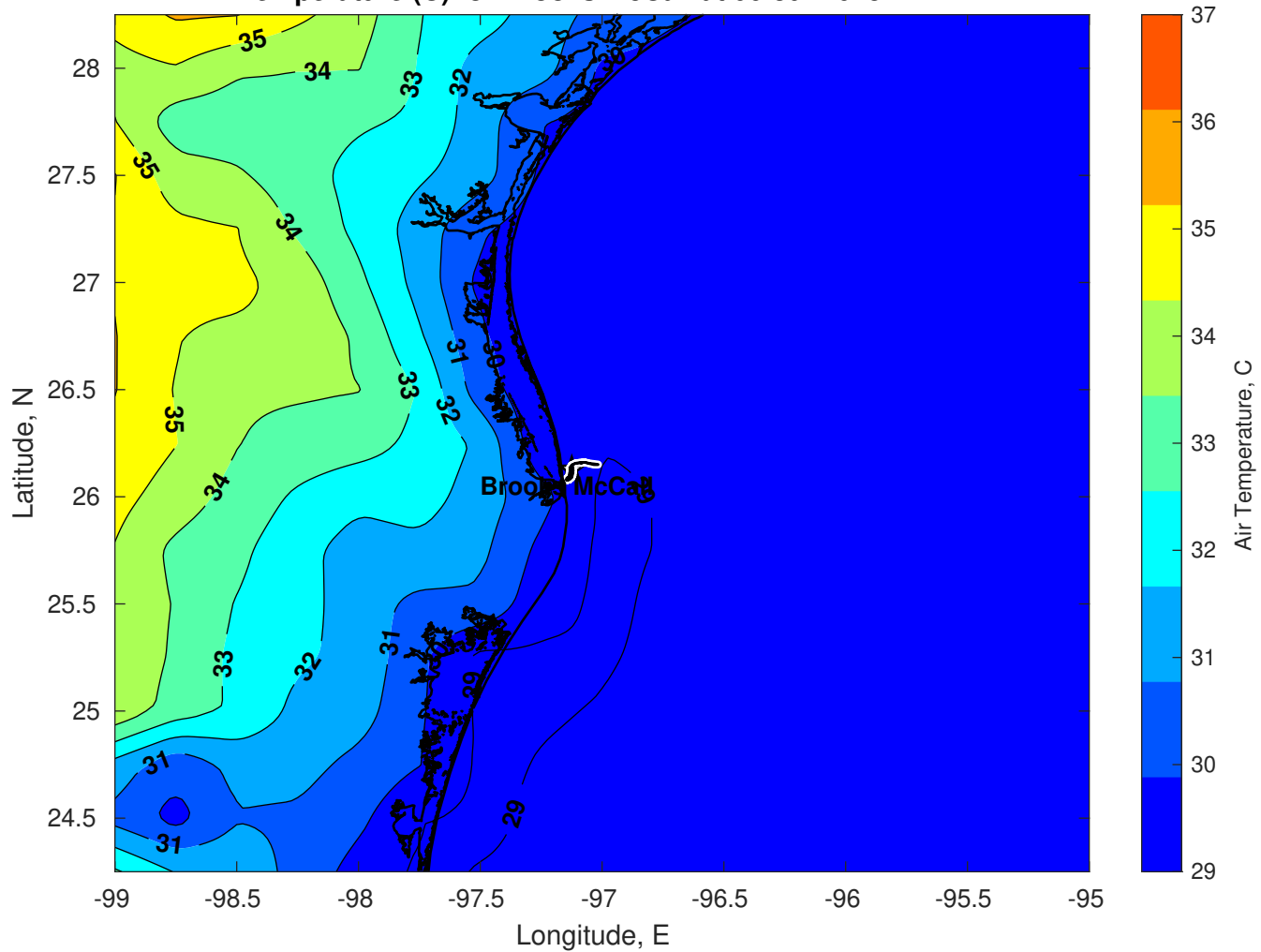
Air Temperature (C) for Brooks McCall at 06-Jul-2025
