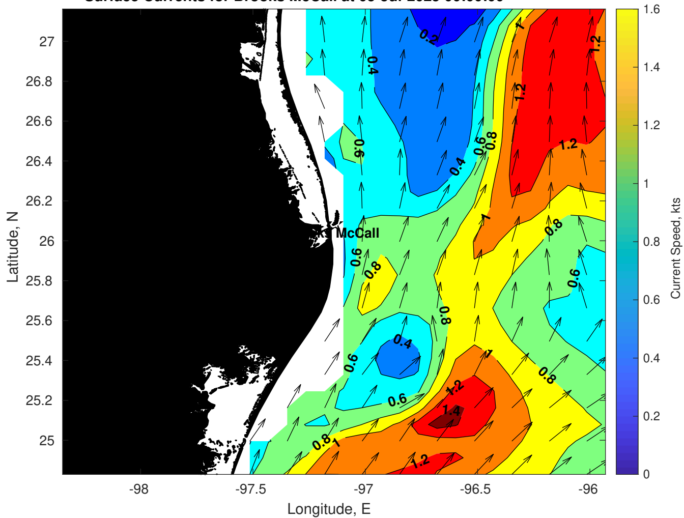
Surface Currents for Brooks McCall at 05-Jul-2025 00:00:00
