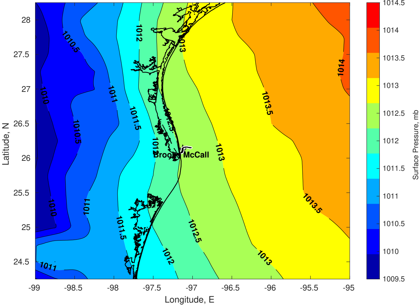
Surface Pressure (mb) for Brooks McCall at 07-Jul-2025 00:00:00
