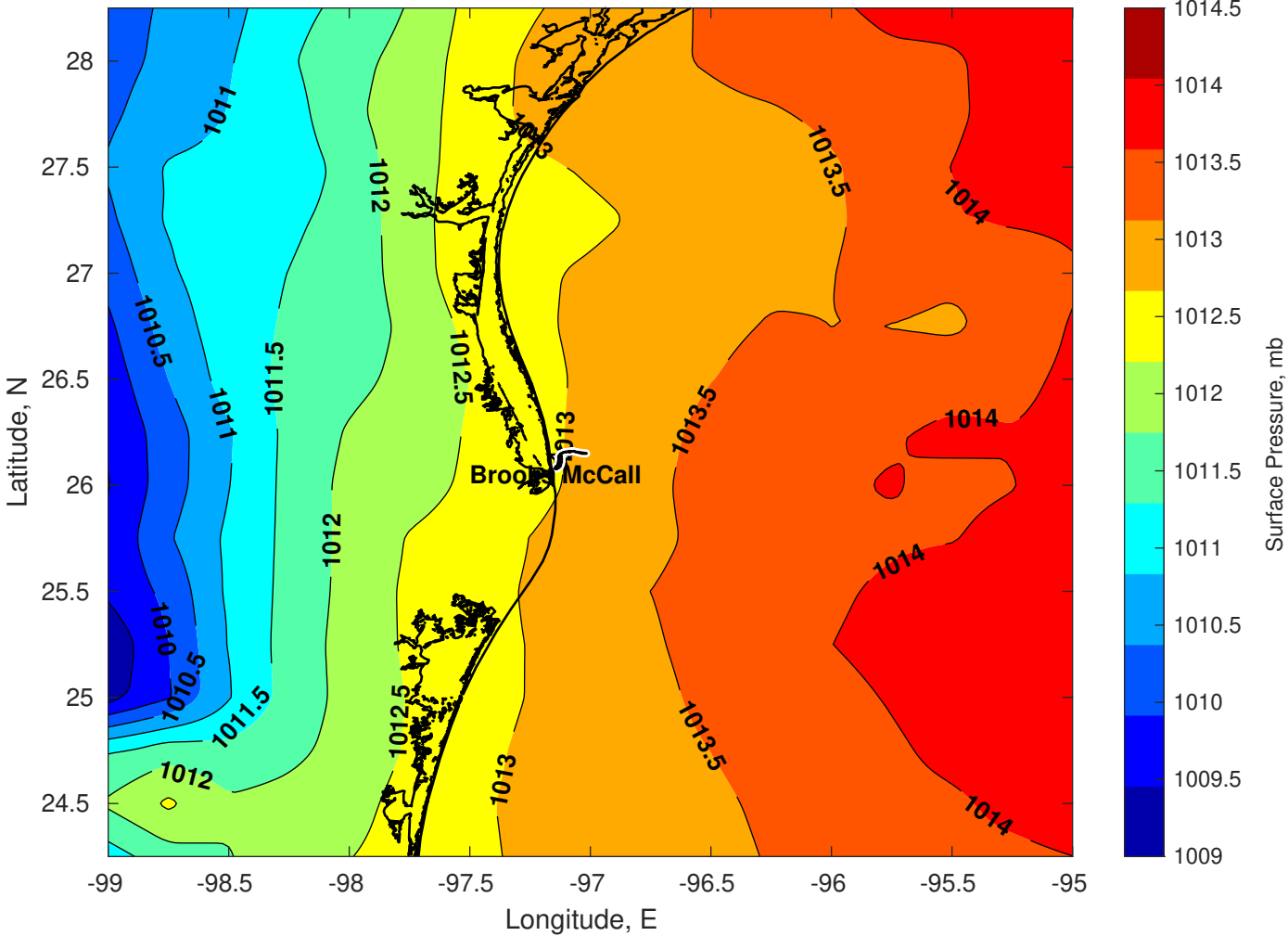
Surface Pressure (mb) for Brooks McCall at 06-Jul-2025 00:00:00
