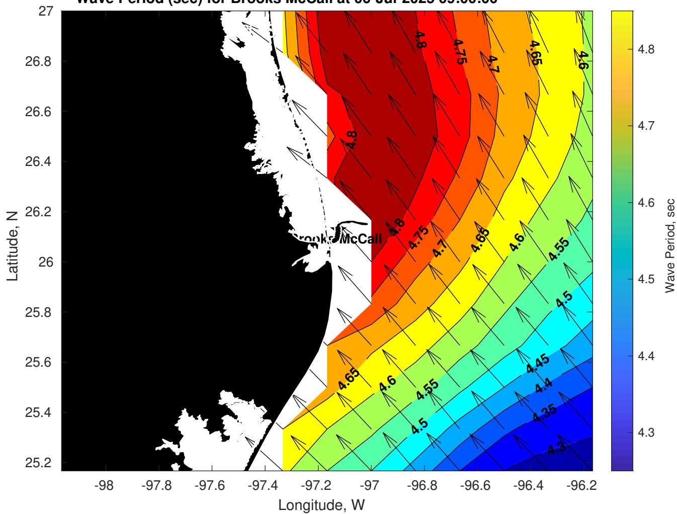
Wave Period (sec) for Brooks McCall at 06-Jul-2025 09:00:00
