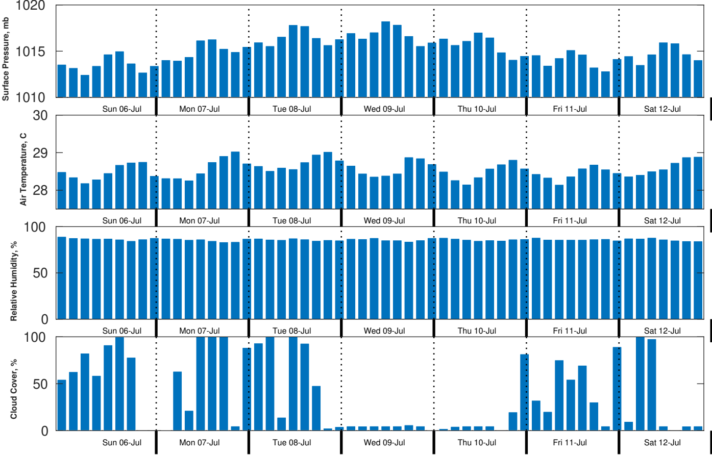
Met Forecast for Brooks McCall from 06-Jul-2025 00:00:00 to 13-Jul-2025 00:00:00
