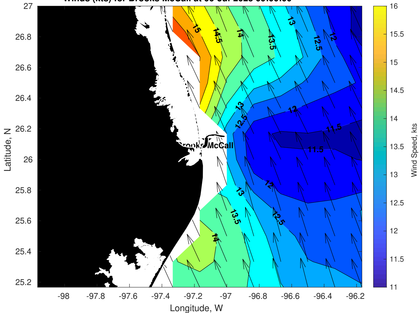
Winds (kts) for Brooks McCall at 06-Jul-2025 09:00:00
