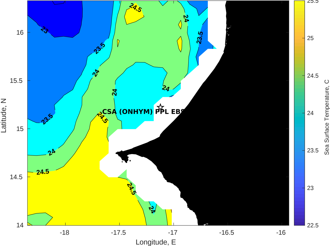
SST for CSA (ONHYM) PPL EBS - Senegal at 07-Jun-2025 00:00:00
