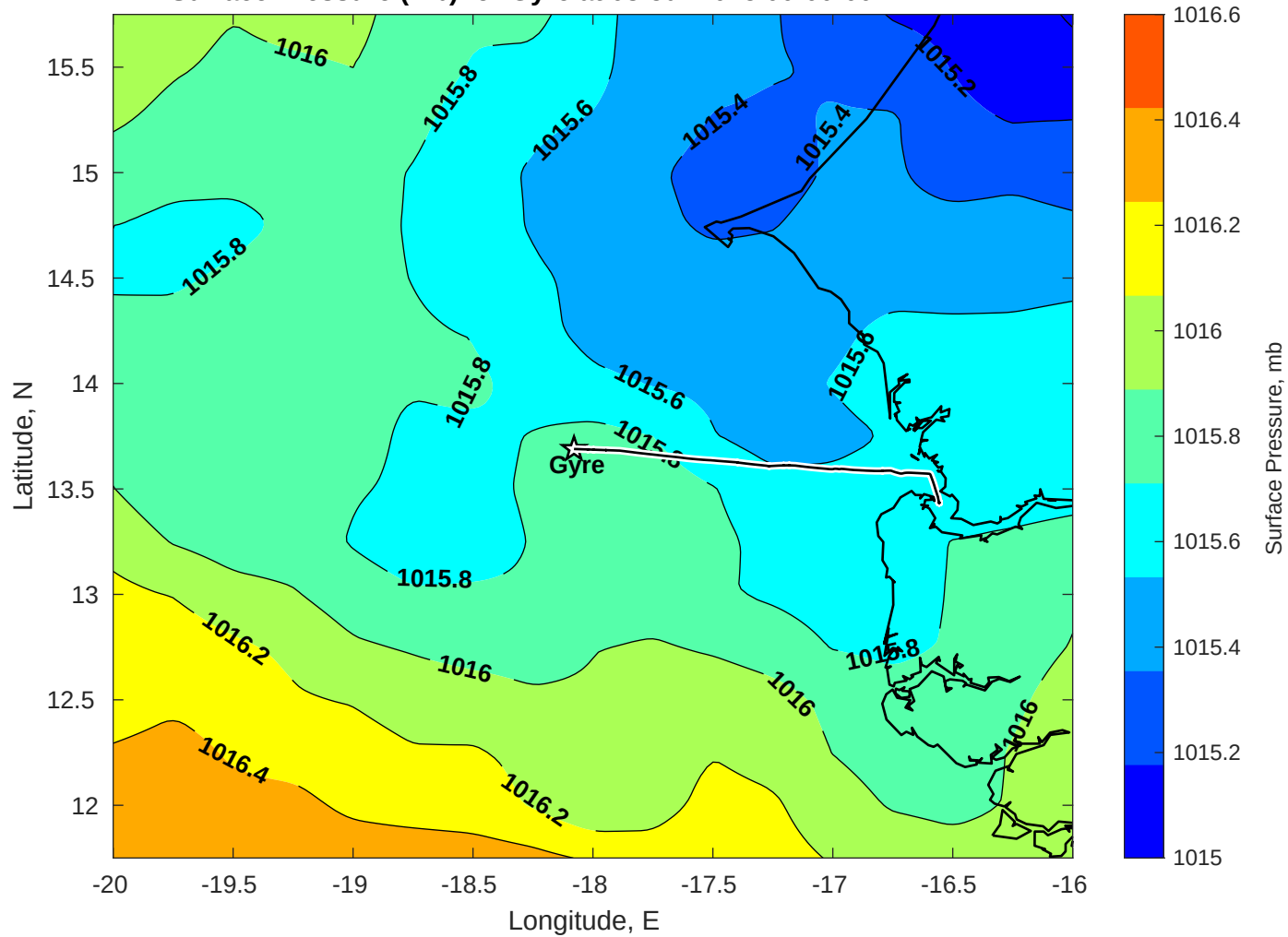
Surface Pressure (mb) for Gyre at 08-Jul-2025 00:00:00
