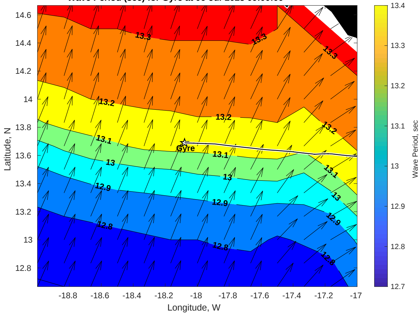
Wave Period (sec) for Gyre at 06-Jul-2025 09:00:00
