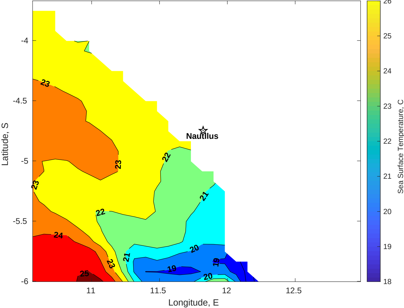
SST for Nautilus at 05-Jul-2025 00:00:00
