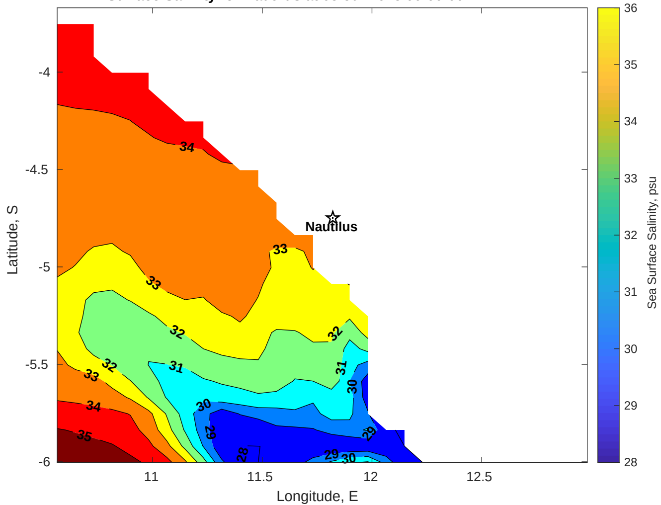
Surface Salinity for Nautilus at 05-Jul-2025 00:00:00
