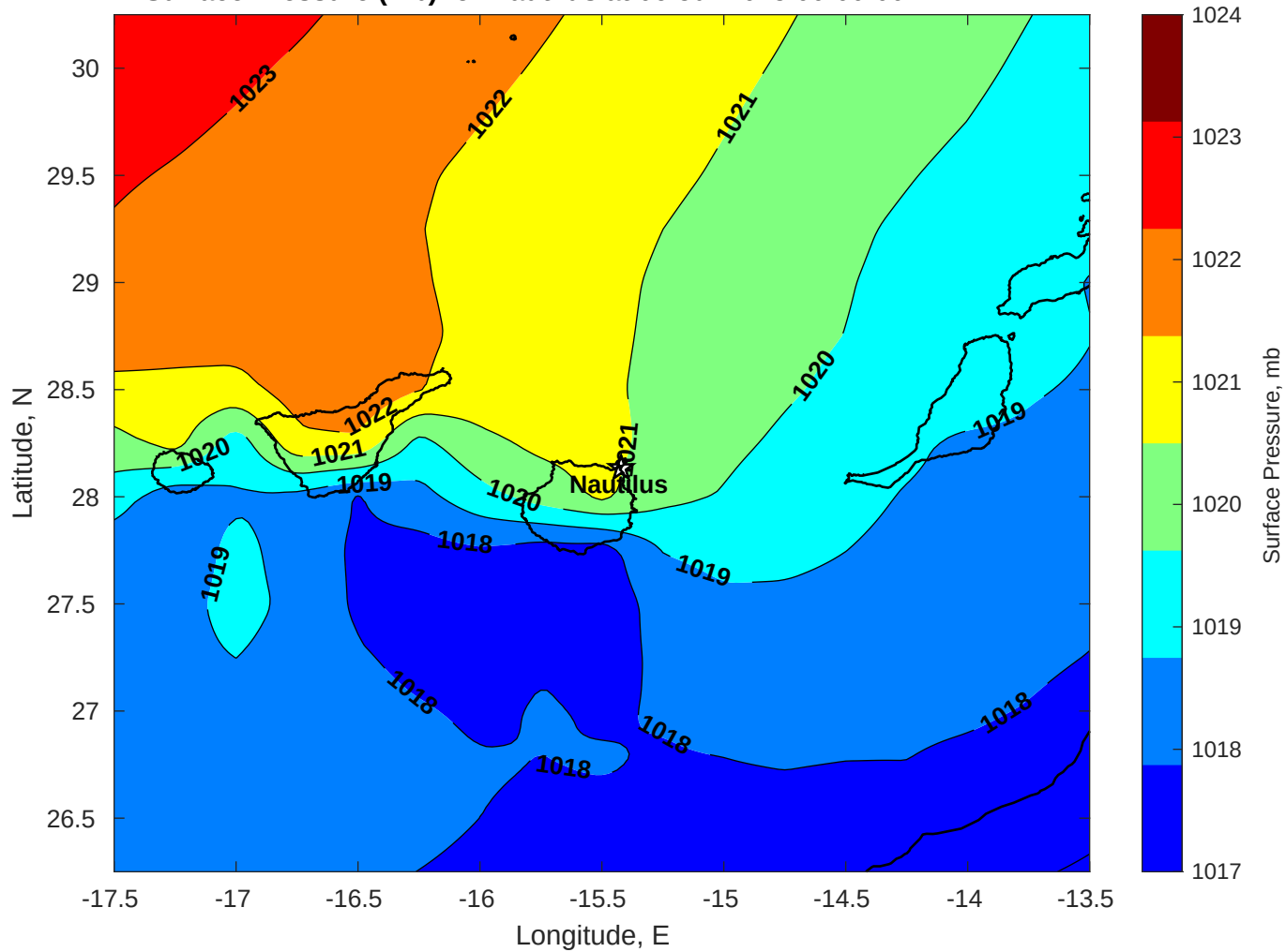
Surface Pressure (mb) for Nautilus at 06-Jul-2025 00:00:00
