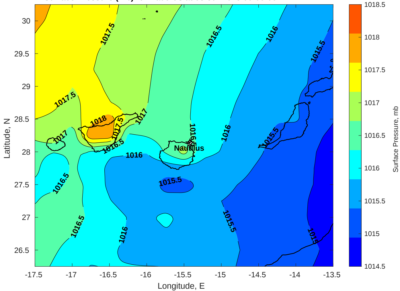
Surface Pressure (mb) for Nautilus at 08-Jul-2025 00:00:00
