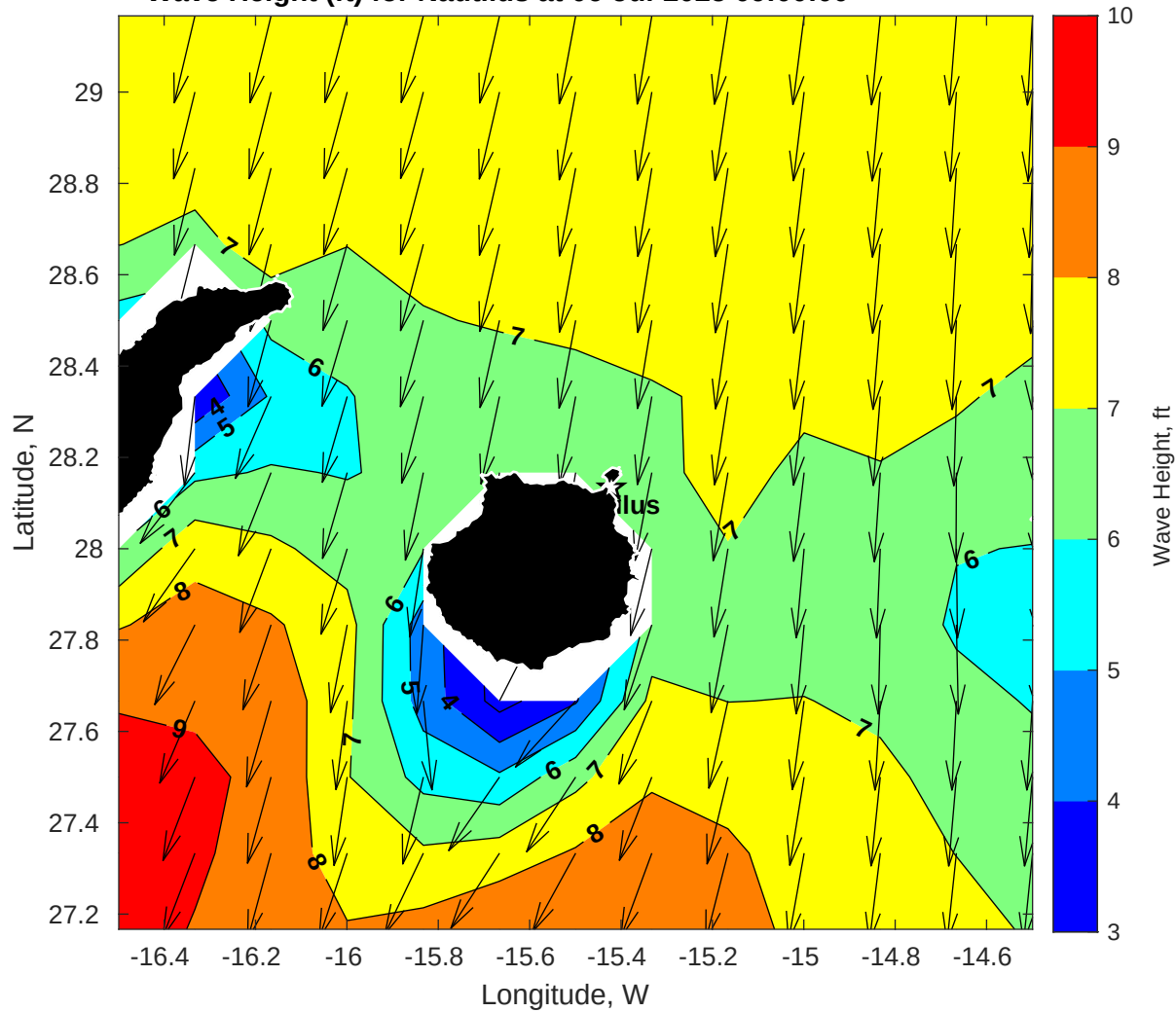
Wave Height (ft) for Nautilus at 06-Jul-2025 09:00:00
