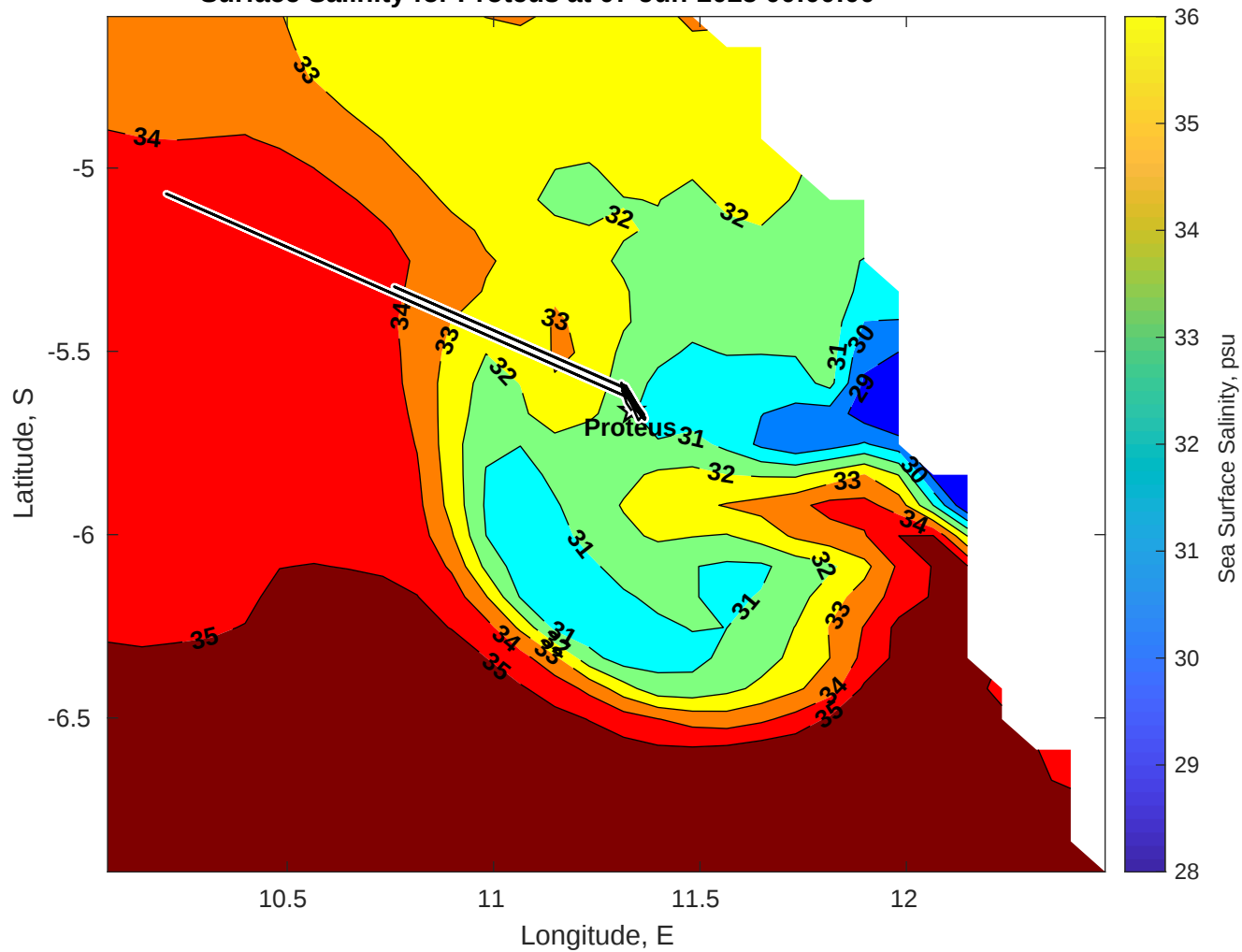
Surface Salinity for Proteus at 07-Jun-2025 00:00:00
