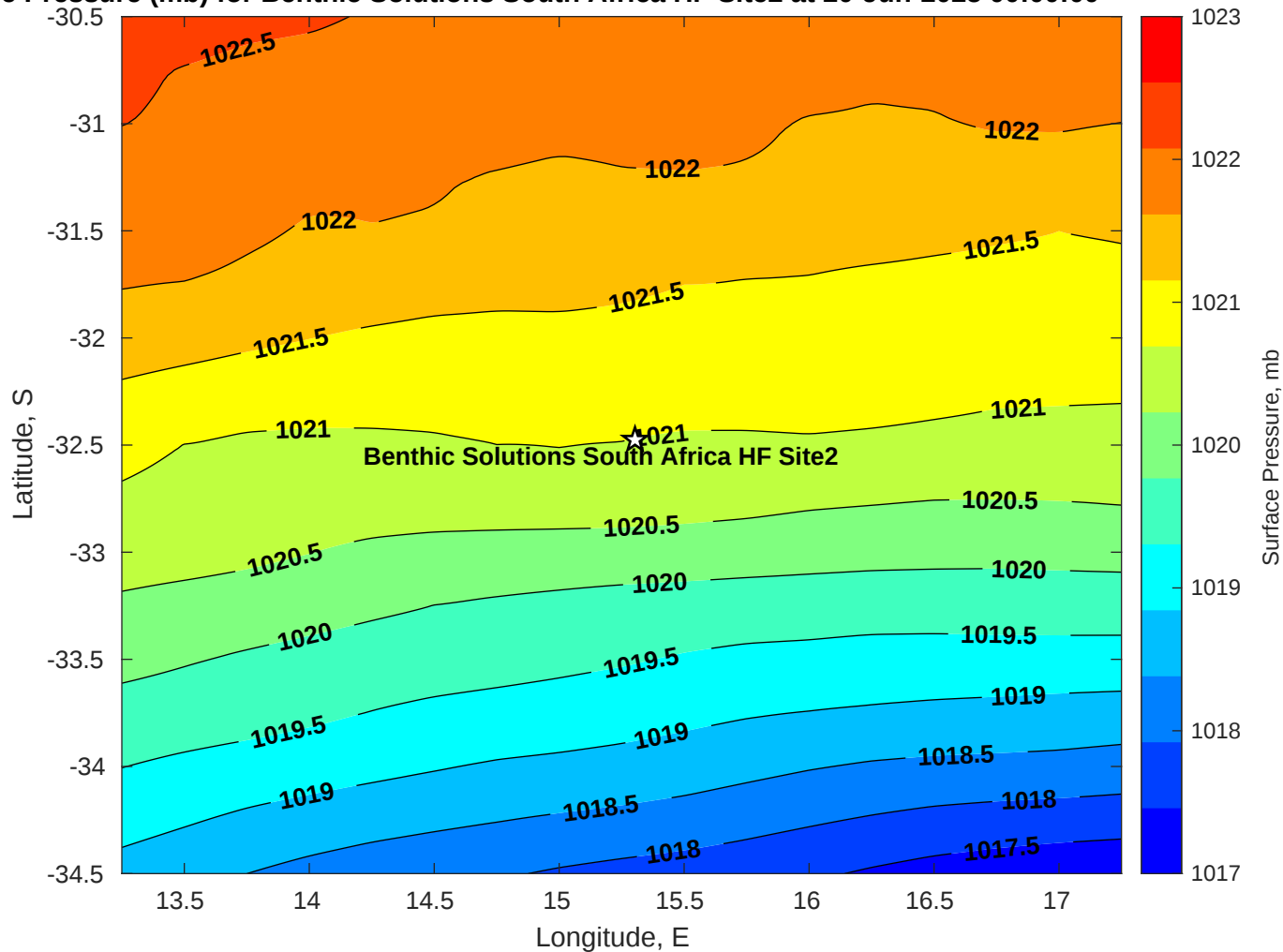
Surface Pressure (mb) for Benthic Solutions South Africa HF Site2 at 20-Jun-2025 00:00:00
