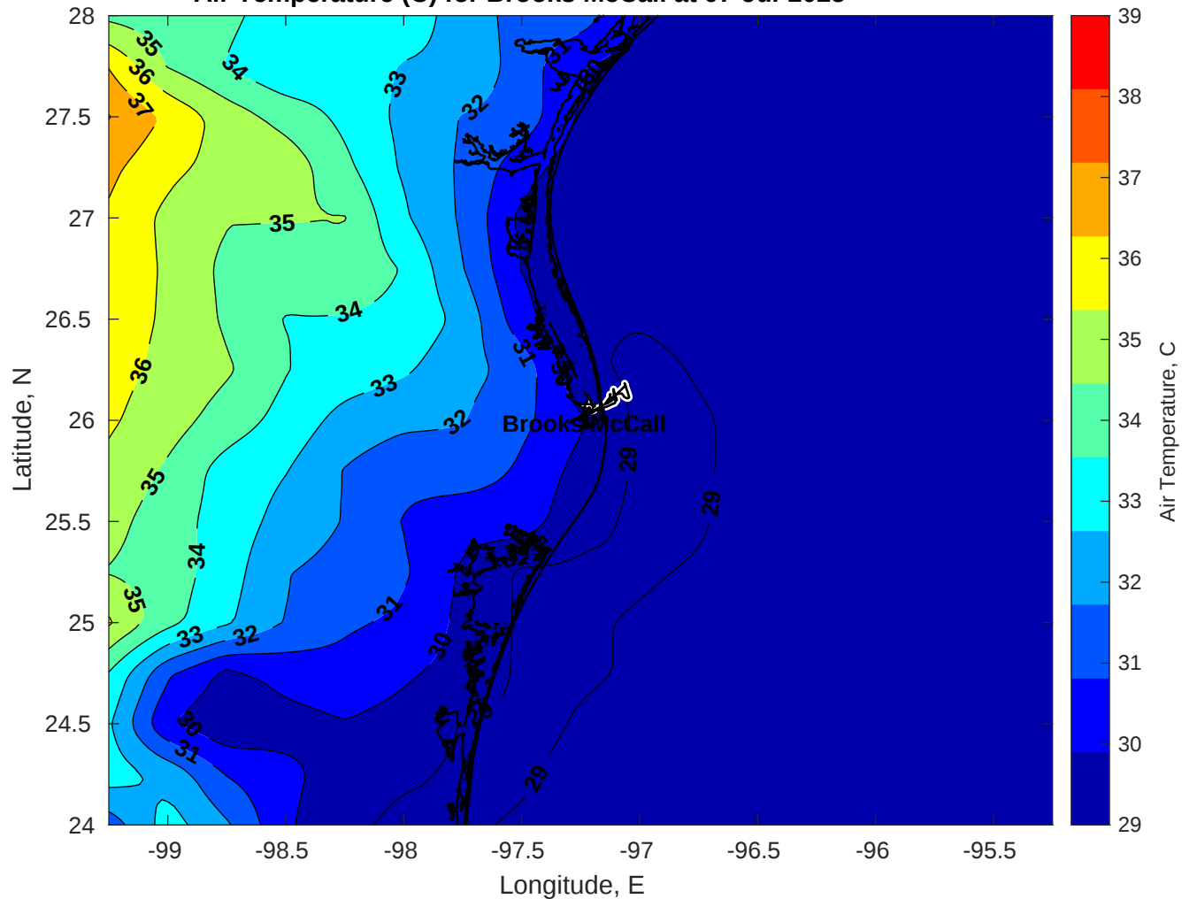
Air Temperature (C) for Brooks McCall at 07-Jul-2025
