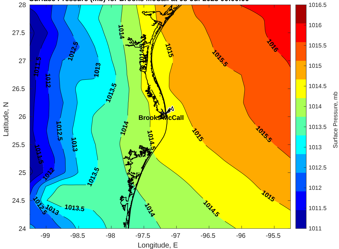
Surface Pressure (mb) for Brooks McCall at 08-Jul-2025 00:00:00
