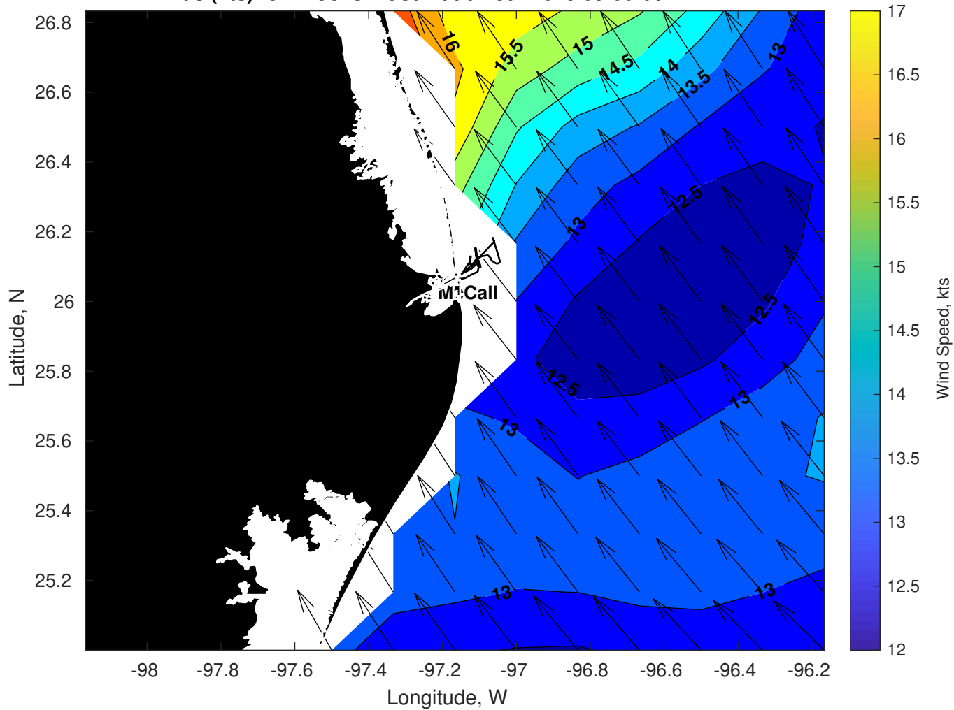
Winds (kts) for Brooks McCall at 07-Jul-2025 09:00:00
