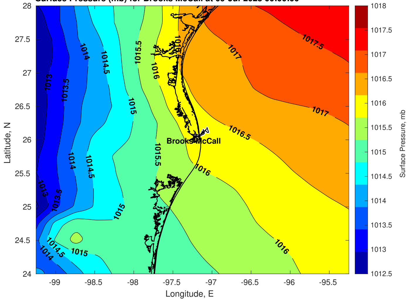
Surface Pressure (mb) for Brooks McCall at 09-Jul-2025 00:00:00
