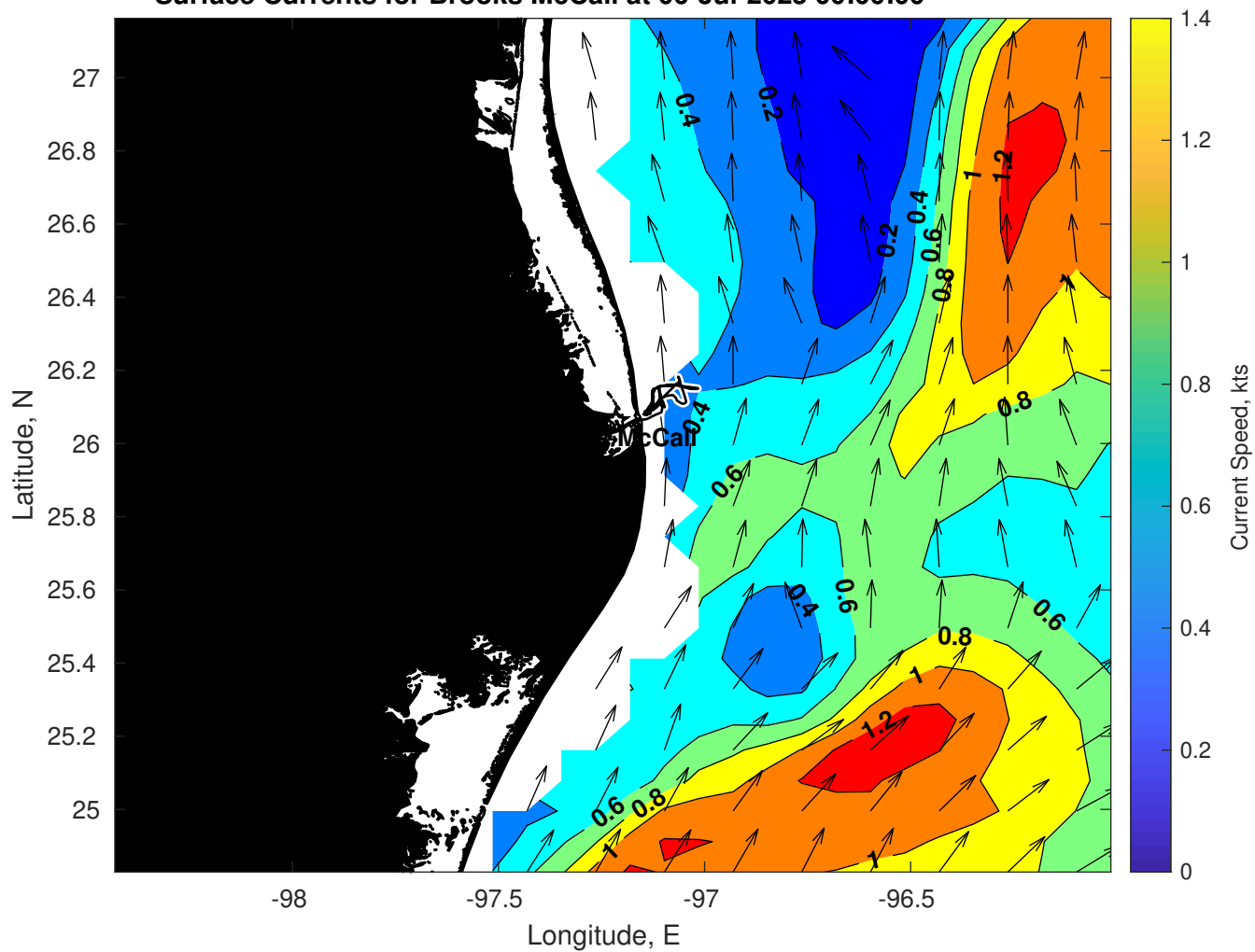
Surface Currents for Brooks McCall at 06-Jul-2025 00:00:00
