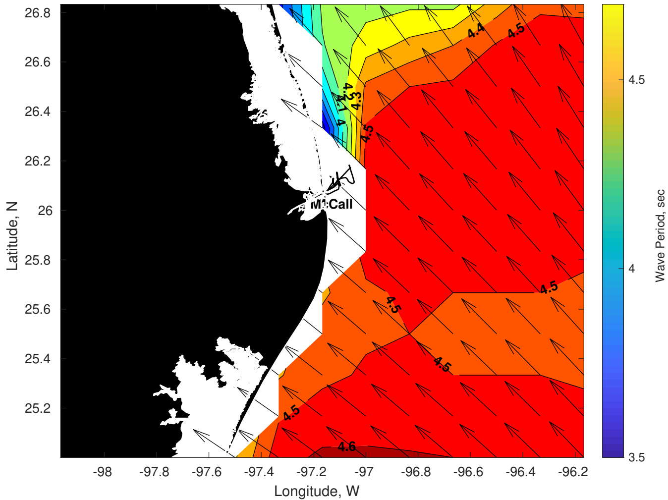
Wave Period (sec) for Brooks McCall at 07-Jul-2025 09:00:00
