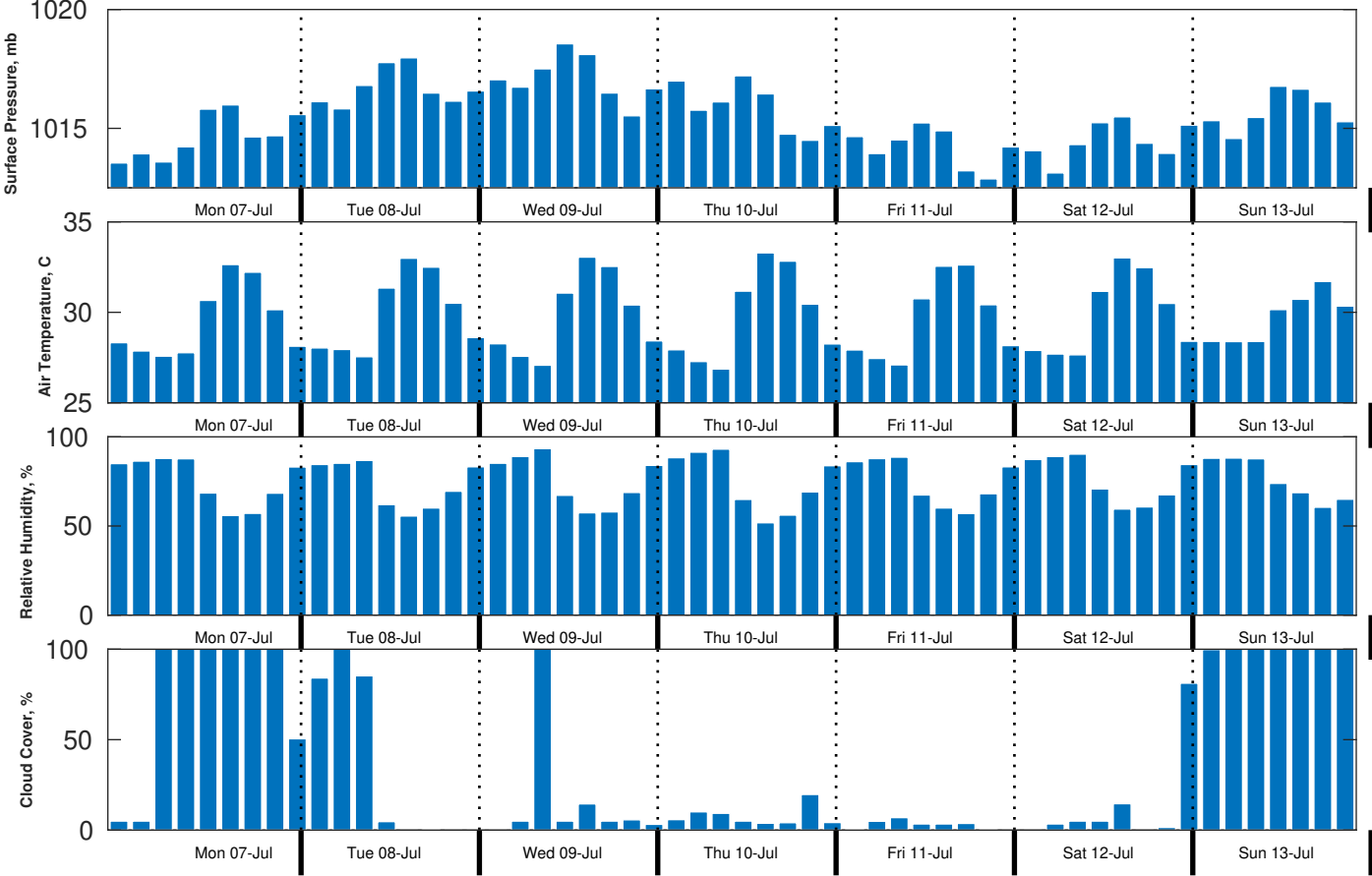
Met Forecast for Brooks McCall from 07-Jul-2025 00:00:00 to 14-Jul-2025 00:00:00
