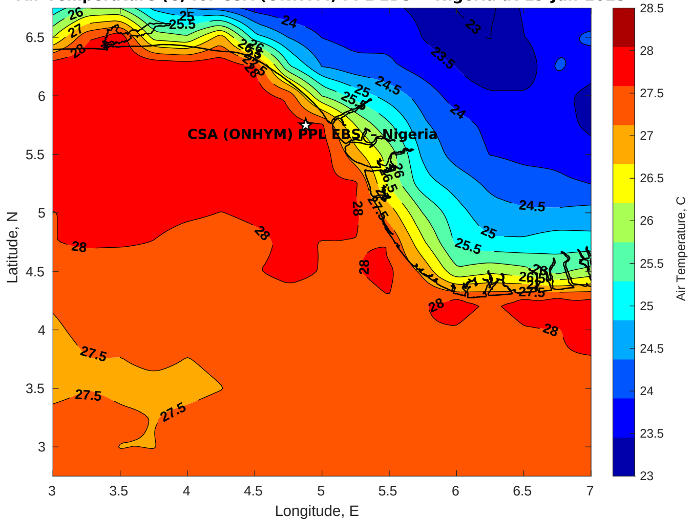
Air Temperature (C) for CSA (ONHYM) PPL EBS - Nigeria at 19-Jun-2025
