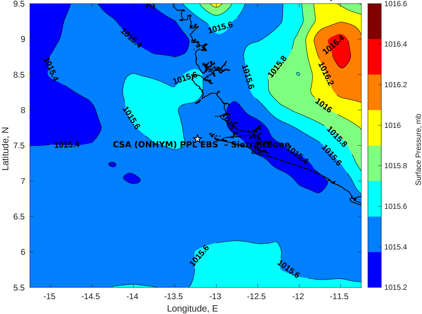
Surface Pressure (mb) for CSA (ONHYM) PPL EBS - Sierra Leone at 21-Jun-2025 00:00:00
