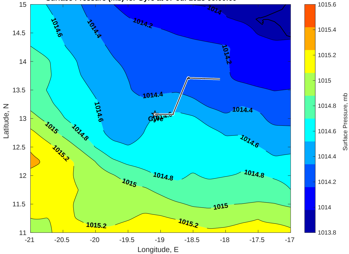
Surface Pressure (mb) for Gyre at 07-Jul-2025 00:00:00
