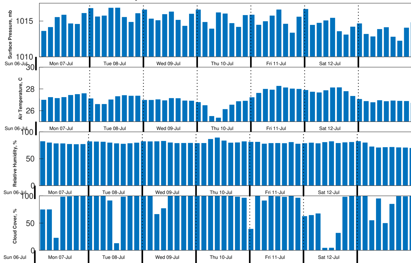
Met Forecast for Gyre from 06-Jul-2025 23:00:00 to 13-Jul-2025 23:00:00
