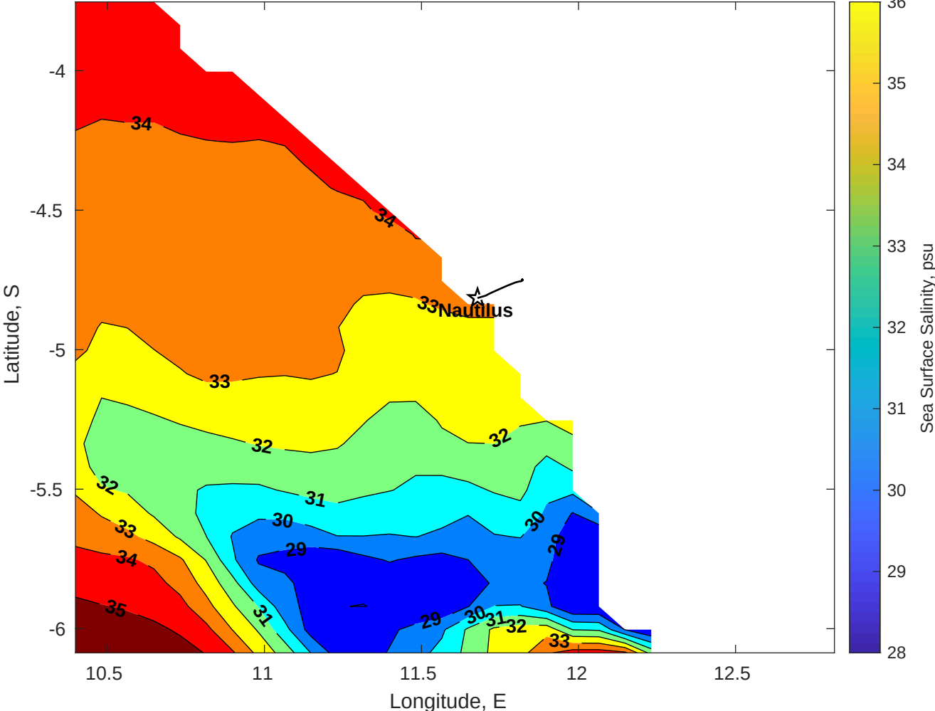
Surface Salinity for Nautilus at 06-Jul-2025 00:00:00
