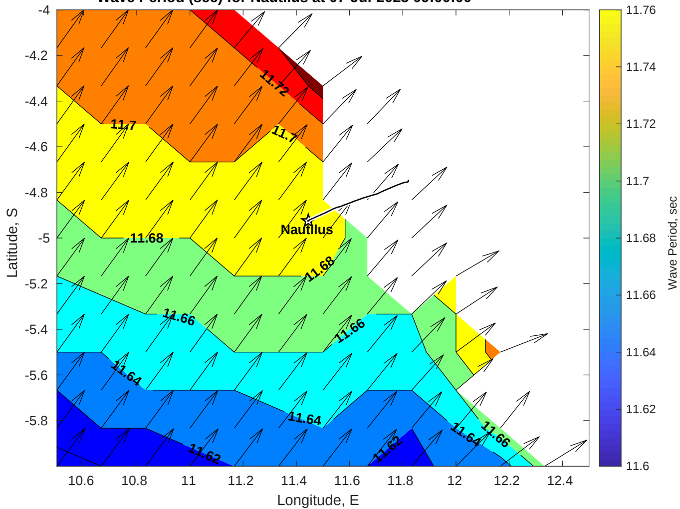
Wave Period (sec) for Nautilus at 07-Jul-2025 09:00:00
