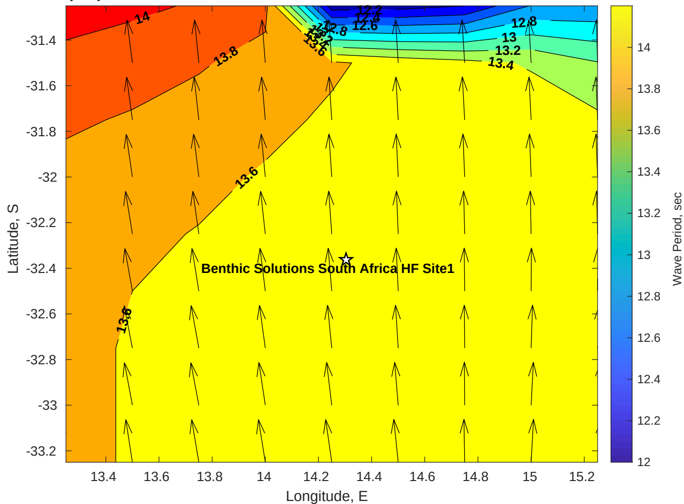
Wave Period (sec) for Benthic Solutions South Africa HF Site1 at 08-Jul-2025 09:00:00
