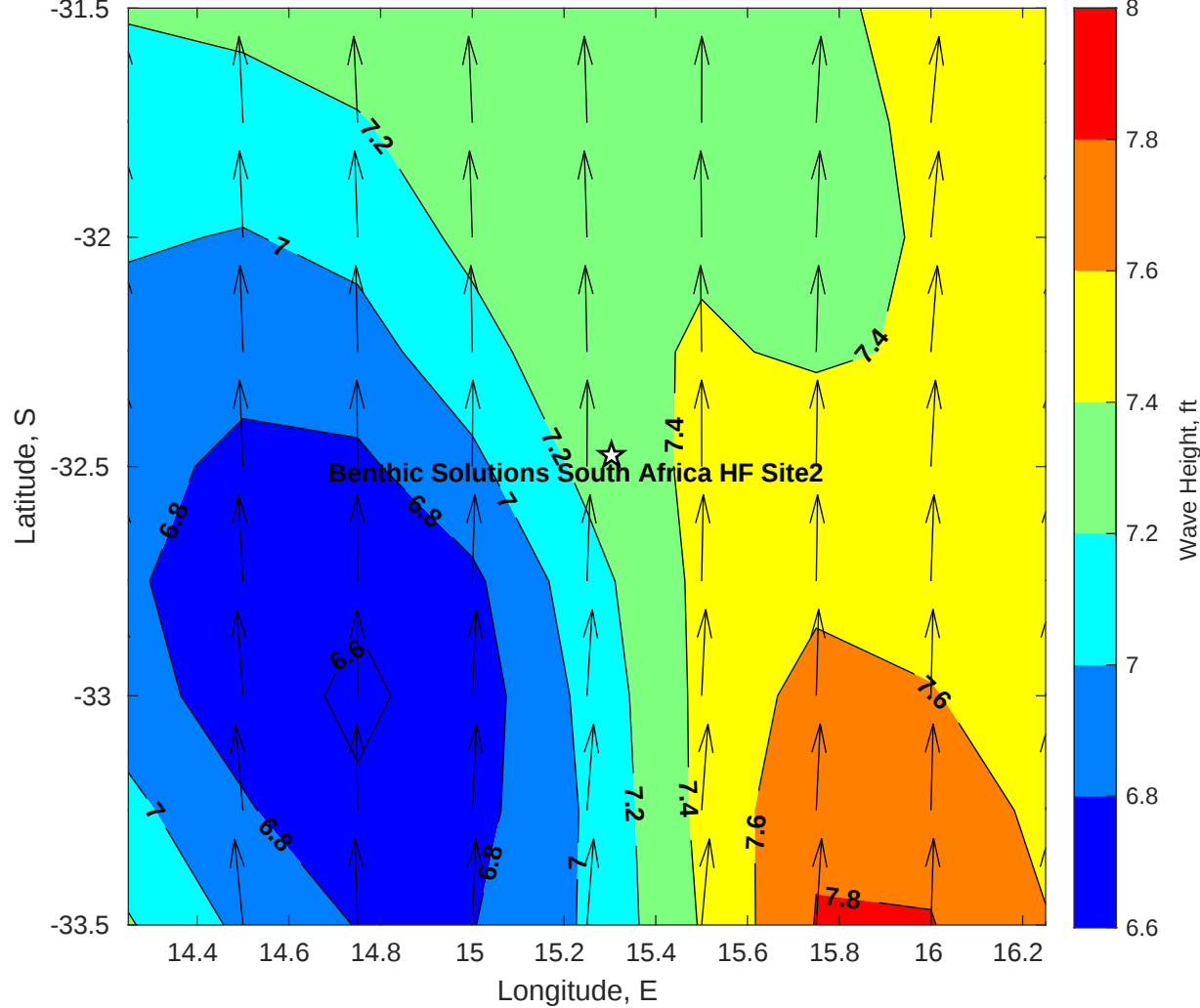
Wave Height (ft) for Benthic Solutions South Africa HF Site2 at 08-Jul-2025 09:00:00
