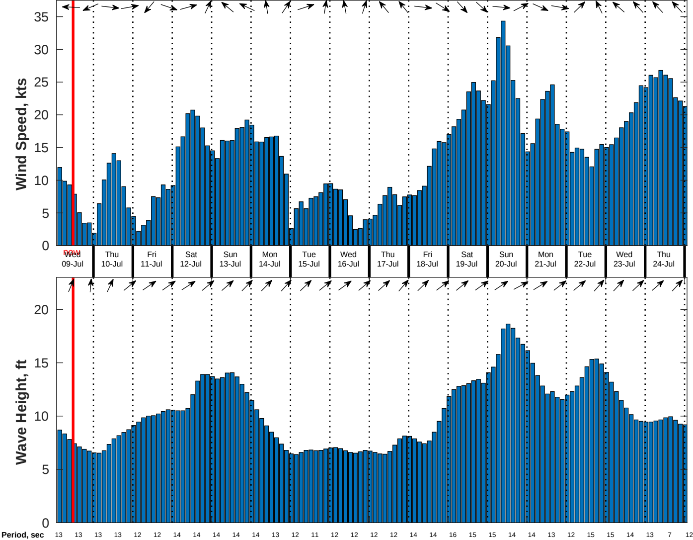
Wind & Wave Forecast for Benthic Solutions South Africa HF Site3 from 08-Jul-2025 02:00:00 to 24-Jul-2025 02:00:00
