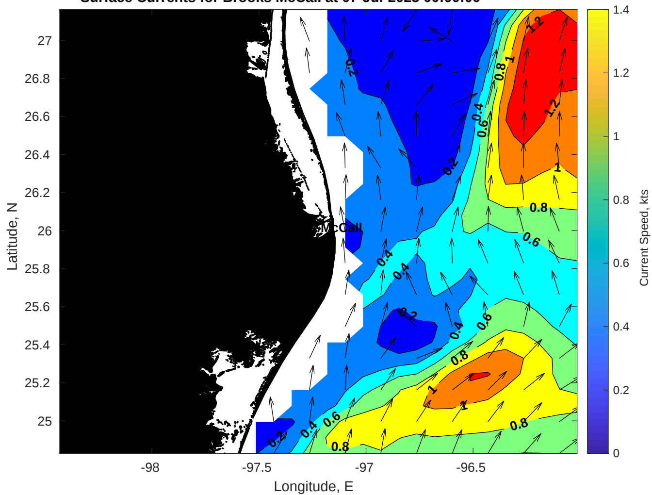
Surface Currents for Brooks McCall at 07-Jul-2025 00:00:00
