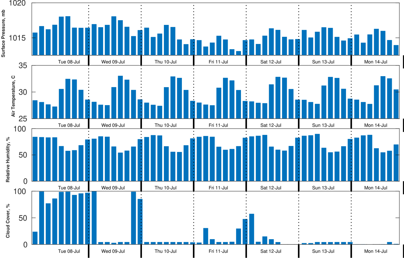
Met Forecast for Brooks McCall from 08-Jul-2025 00:00:00 to 15-Jul-2025 00:00:00
