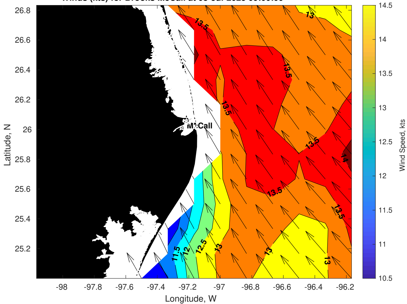
Winds (kts) for Brooks McCall at 08-Jul-2025 09:00:00
