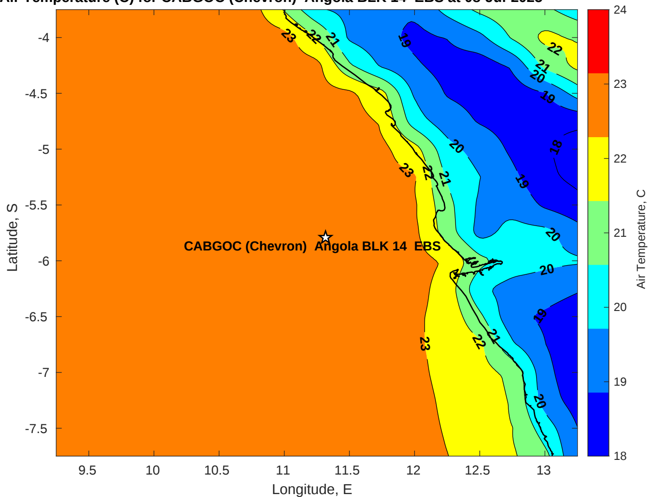
Air Temperature (C) for CABGOC (Chevron) Angola BLK 14 EBS at 08-Jul-2025
