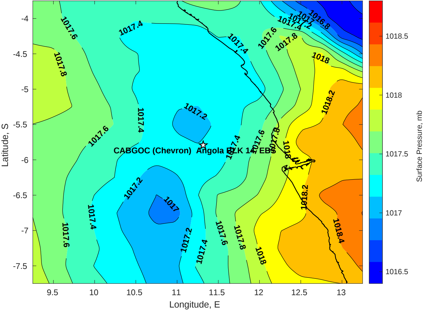
Surface Pressure (mb) for CABGOC (Chevron) Angola BLK 14 EBS at 09-Jul-2025 00:00:00
