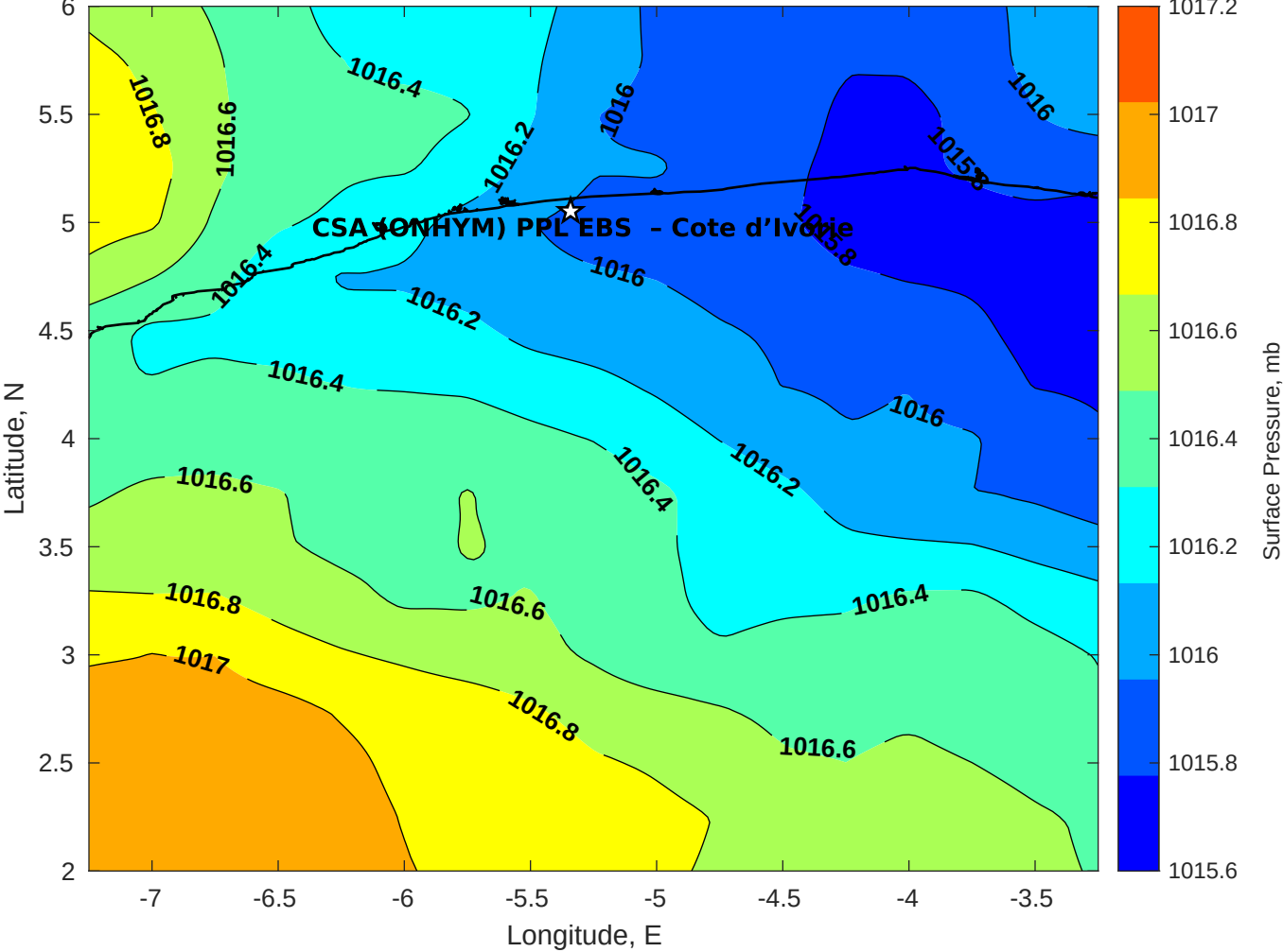
Surface Pressure (mb) for CSA (ONHYM) PPL EBS - Cote d'Ivoire at 08-Jul-2025 00:00:00
