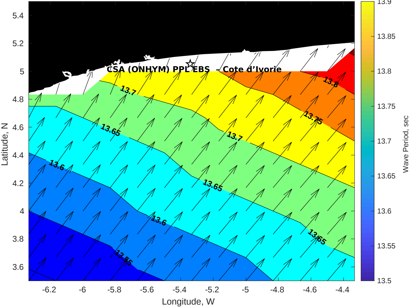
Wave Period (sec) for CSA (ONHYM) PPL EBS - Cote d'Ivoire at 08-Jul-2025 09:00:00
