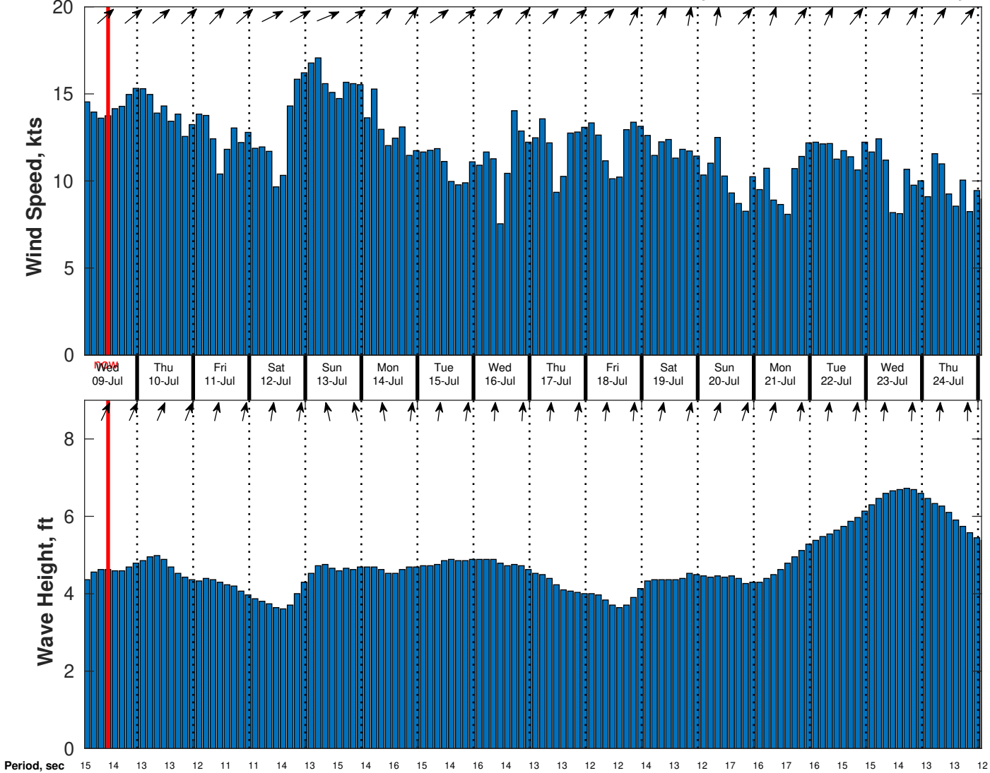
Wind & Wave Forecast for CSA (ONHYM) PPL EBS - Cote d'Ivoire from 08-Jul-2025 01:00:00 to 24-Jul-2025 01:00:00
