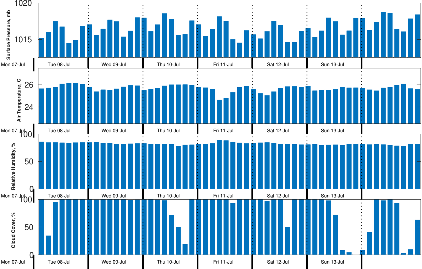
Met Forecast for CSA (ONHYM) PPL EBS - Cote d'Ivoire from 08-Jul-2025 00:00:00 to 15-Jul-2025 00:00:00
