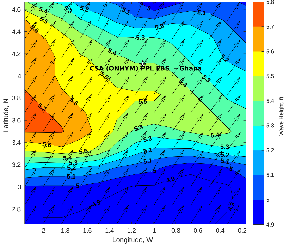
Wave Height (ft) for CSA (ONHYM) PPL EBS - Ghana at 08-Jul-2025 09:00:00
