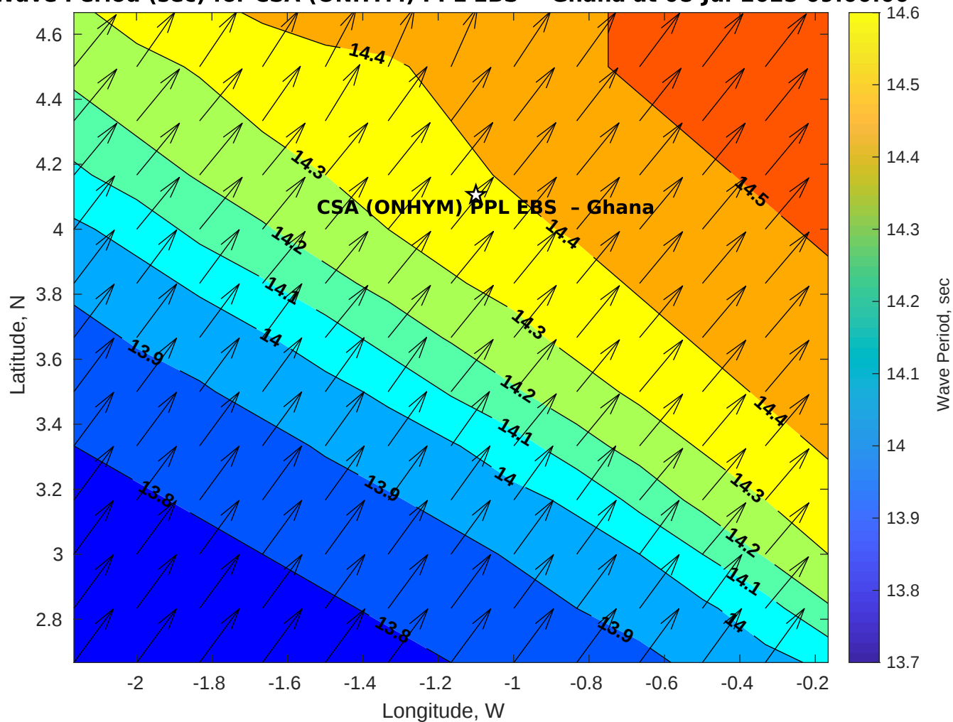
Wave Period (sec) for CSA (ONHYM) PPL EBS - Ghana at 08-Jul-2025 09:00:00
