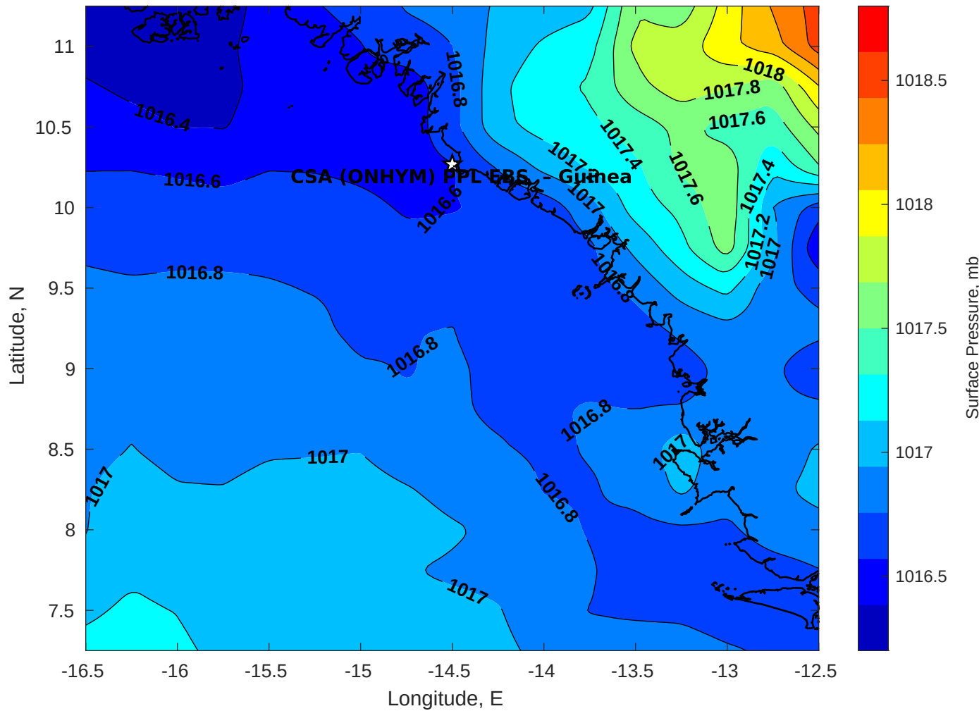
Surface Pressure (mb) for CSA (ONHYM) PPL EBS - Guinea at 08-Jul-2025 00:00:00
