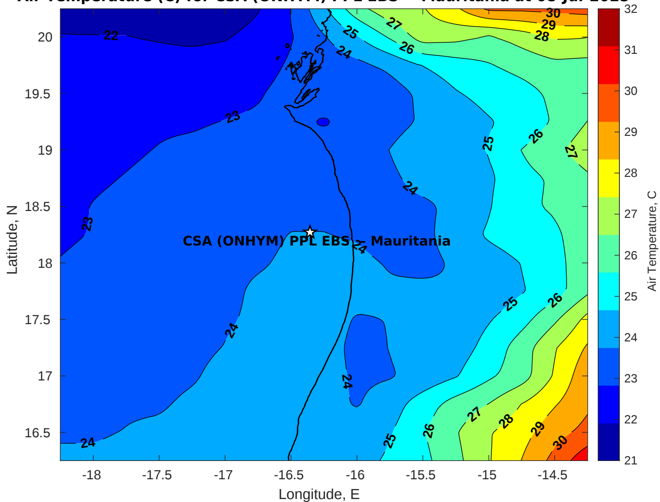
Air Temperature (C) for CSA (ONHYM) PPL EBS - Mauritania at 08-Jul-2025
