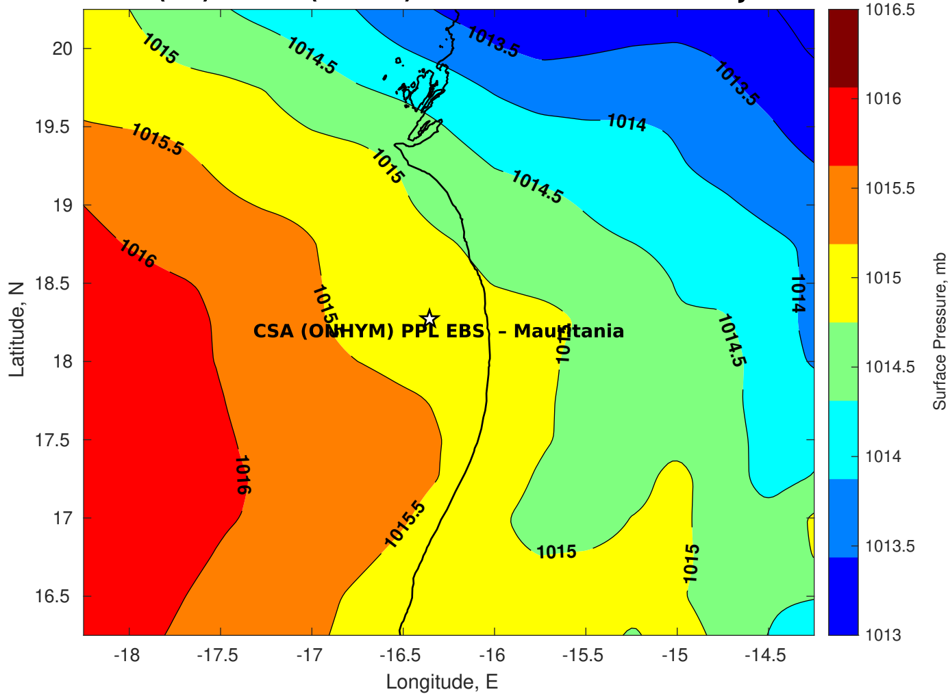
Surface Pressure (mb) for CSA (ONHYM) PPL EBS - Mauritania at 08-Jul-2025 00:00:00
