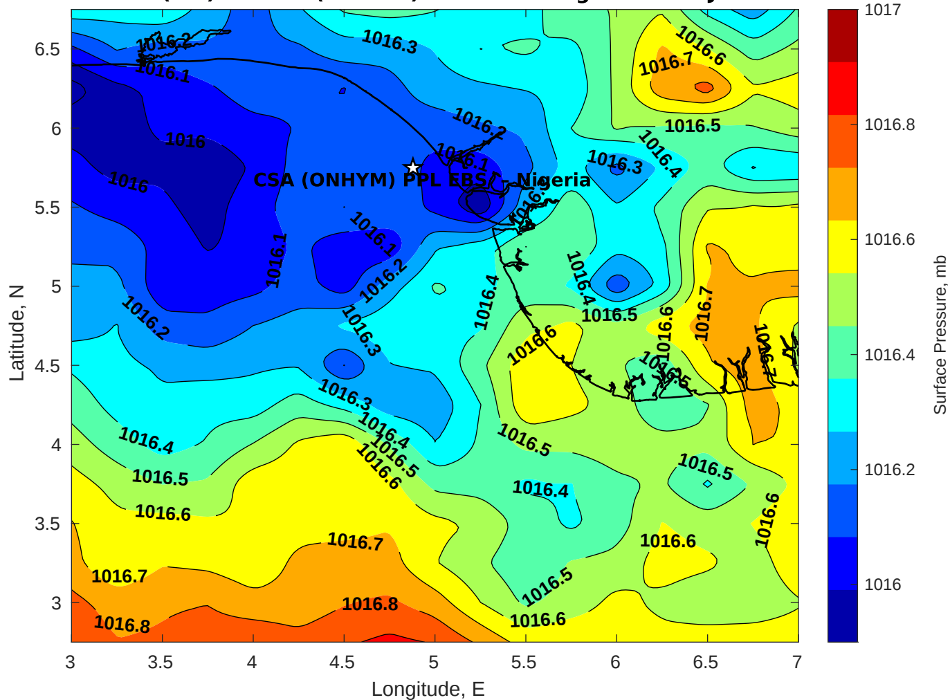
Surface Pressure (mb) for CSA (ONHYM) PPL EBS - Nigeria at 09-Jul-2025 00:00:00
