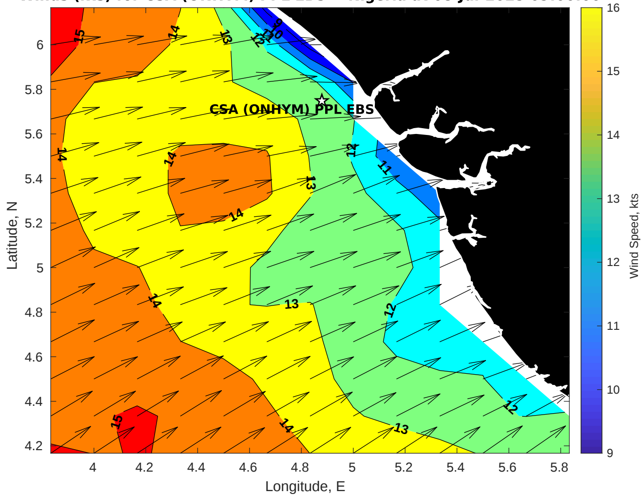
Winds (kts) for CSA (ONHYM) PPL EBS - Nigeria at 08-Jul-2025 09:00:00
