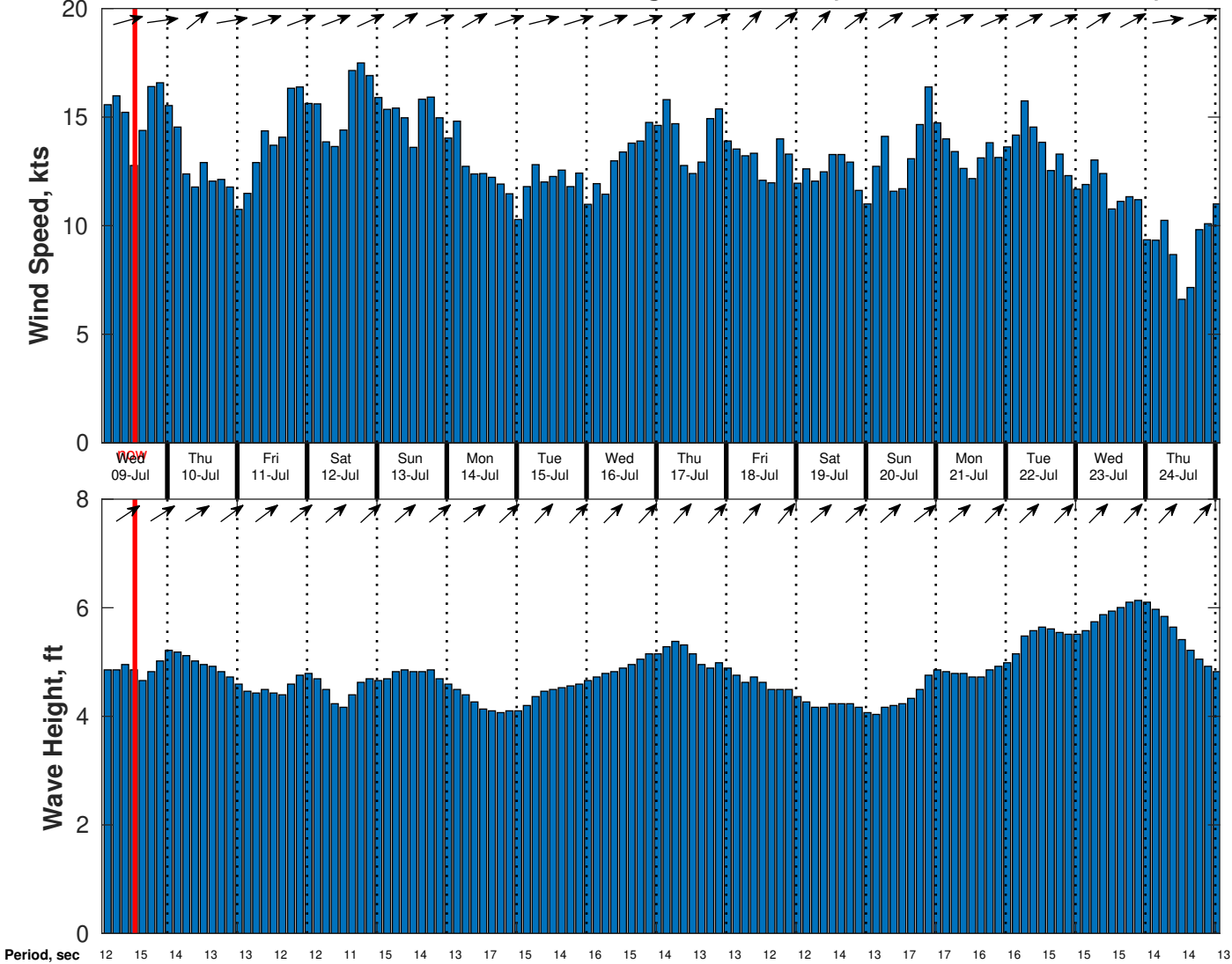
Wind & Wave Forecast for CSA (ONHYM) PPL EBS - Nigeria from 08-Jul-2025 02:00:00 to 24-Jul-2025 02:00:00
